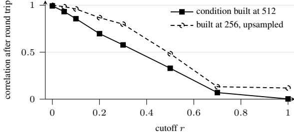
Figure 7: Correlation between the condition fed to the autoencoder and the same condition re-extracted after an encode-decode round trip, 24 images chosen by [AUTHOR-INPUT A37]. Above r \approx 0.5 the condition is effectively gone. Building the condition at 256 and upsampling puts the structure at lower absolute frequency and preserves far more, which is why comparisons against older pipelines need the source resolution stated.
