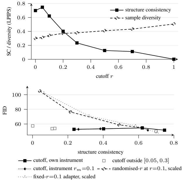
Figure 4: Top: structure consistency and sample diversity against the cutoff (values of Table 2, which gives SEM and seed sd). Bottom: FID against structure consistency, one FID estimate per point. Filled squares: the cutoff sweep scored at its own cutoff on r \in [0.05, 0.3] ; open grey squares: the same sweep outside that range. Diamonds: the same generations re-scored with the instrument fixed at r_m=0.1 . Circles and triangles: the randomised- r and fixed- r=0.1 adapters scaled at r=0.1 , which already use r_m=0.1 . On that one instrument the cutoff r=0.3 reaches 0.2599 at FID 52.77, while scale 0.50 reaches 0.2146 at FID 76.46. Both panels are plotted directly from the evaluation outputs.
