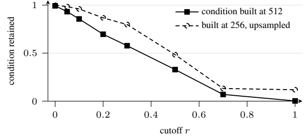
Figure 5: Correlation between the condition fed to the autoencoder and the same condition re-extracted after an encode-decode round trip, 24 images. Above r\approx 0.5 the condition is effectively gone, so an adapter reading the VAE latent cannot recover it. Building the condition at 256 and upsampling puts the structure at lower absolute frequency and preserves far more, which is why comparisons against older pipelines need the source resolution stated.
