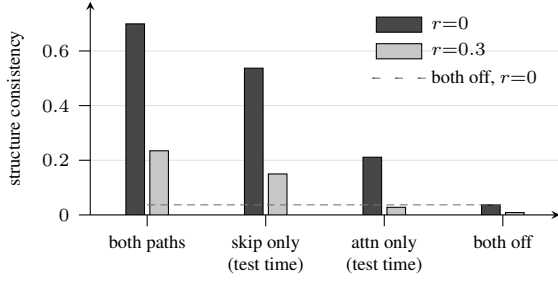
Figure 9: Both injection paths on, then each alone, then neither. The skip residuals carry most of the structure signal; cross-attention alone recovers little of it, and with both off the model falls to the frozen backbone (FID 120.50 against 50.13 with both paths on; skip only 65.12, attention only 67.07). The dashed line is the both-off control at r=0 . Paths are switched off at test time on the trained main model; the separately trained skip-only model is in Table 7. At r=0 the single-path gains over the control roughly add up to the both-paths gain; at r=0.3 the both-paths gain over the control exceeds the sum of the single-path gains.
