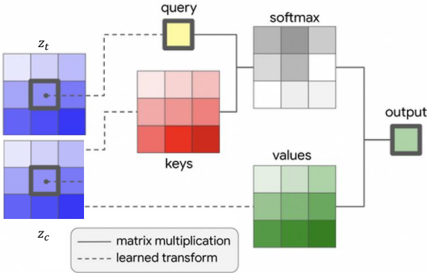
Figure 3: One Stand Alone site. The query is one position of the UNet latent z_t ; the keys and values are the 3 \times 3 neighbourhood of the same position in the condition z_c , so the softmax runs over 9 entries rather than the whole map, and a 1 \times 1 window performs at least as well (Sec. 5.2). W_K , W_V and the zero-initialised per-channel gate are trained; W_Q and the output projection stay frozen. The gated result is added both into the latent — so the text query below sees structure — and to what the layer returns.
