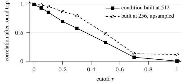
Figure 8: Correlation between the condition fed to the autoencoder and the same condition re-extracted after an encode–decode round trip, the first 24 FFHQ-512 images in file order, which are not the test split. Above r \approx 0.5 the condition is effectively gone. Building the condition at 256 and upsampling puts the structure at lower absolute frequency and preserves far more, which is why comparisons against older pipelines need the source resolution stated.
