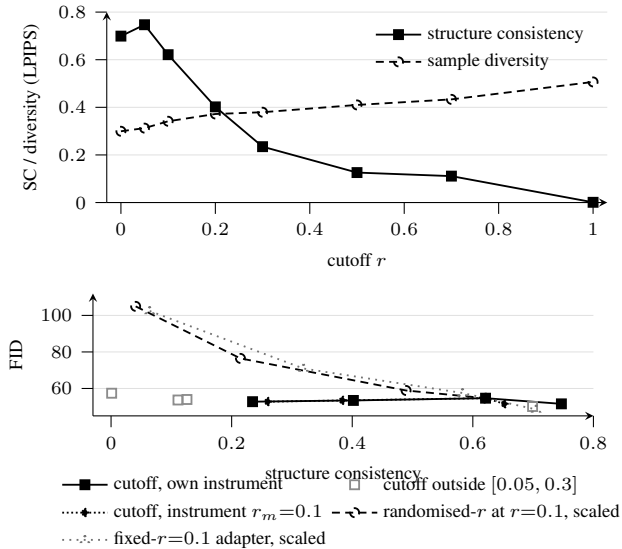
Figure 5: Top: structure consistency and sample diversity against the cutoff (values of Table 2, which gives SEM and seed sd). Bottom: FID against structure consistency, one FID estimate per point. Filled squares: the cutoff sweep scored at its own cutoff on r \in [0.05, 0.3] ; open grey squares: the same sweep outside that range. Diamonds: the same generations re-scored with the instrument fixed at r_m=0.1 . Circles and triangles: the randomised- r and fixed- r=0.1 adapters scaled at r=0.1 , which already use r_m=0.1 . On that one instrument the cutoff r=0.3 reaches 0.2599 at FID 52.77, while scale 0.50 reaches 0.2146 at FID 76.46. Both panels are plotted directly from the evaluation outputs.
