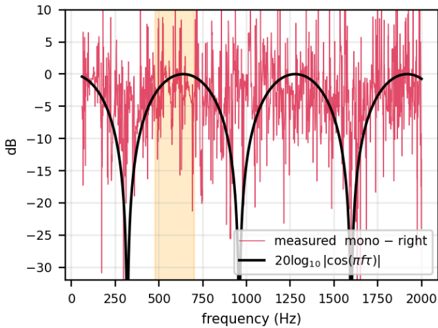
Figure 7: The naive mono downmix relative to the right channel alone, against Equation 27. Shaded: 476–700 Hz, where the comb’s first maximum falls.
