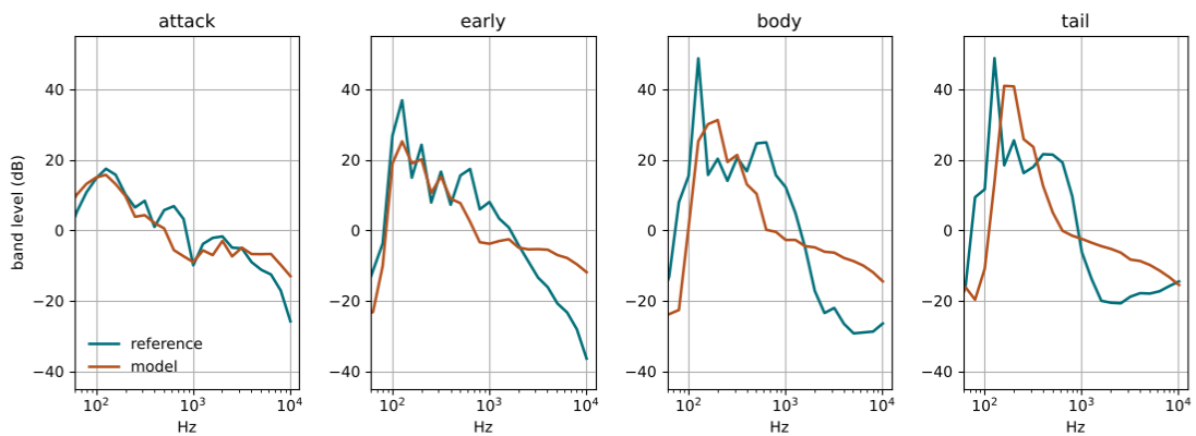
Figure 5: Spectral envelope, window by window. The attack matches closely; the discrepancy appears in the body and tail and is concentrated above 1 kHz, where the model runs 20–30 dB hot.
