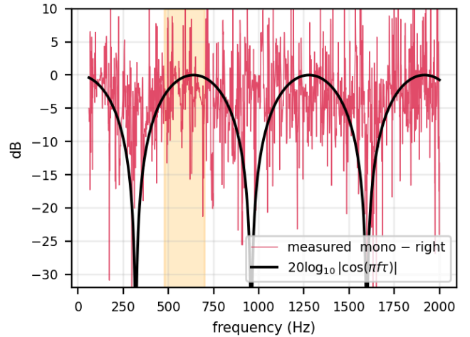
Figure 7: The naive mono downmix relative to the right channel alone, against Equation 21. Shaded: 476–700 Hz, where the comb’s first maximum falls.
