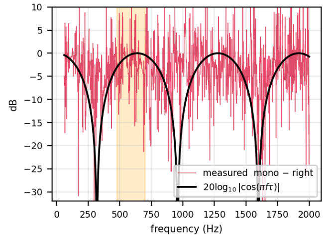
Figure 2: The naive mono downmix relative to the right channel alone, against Equation 1. Shaded: 476–700 Hz, where the comb’s first maximum falls.
