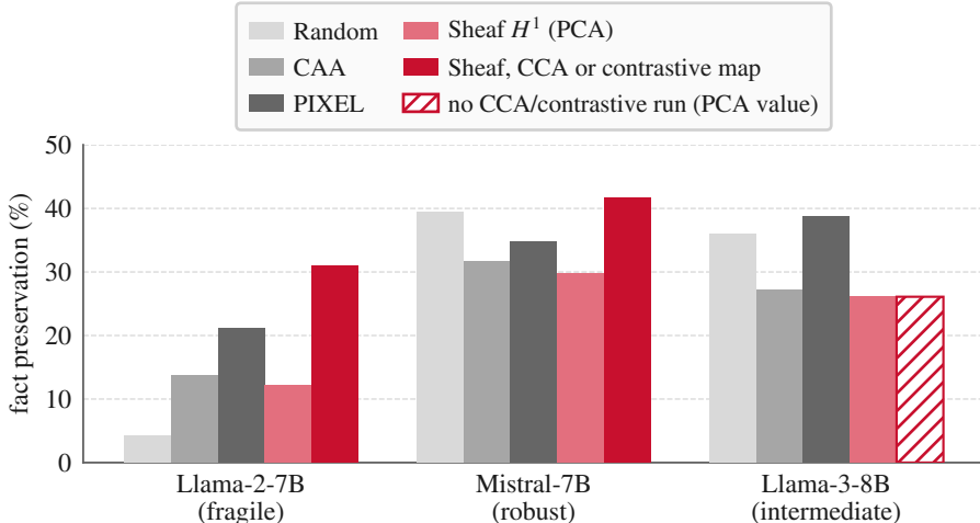
Figure 4: Steering on CounterFact at \alpha = 0.3 ( n = 1000 per model) for the three architectures with a PIXEL run. The hatched bar on Llama-3-8B repeats the PCA H^1 value, since that model has no CCA or contrastive run. On fragile Llama-2-7B, random steering collapses to 4.2% and the contrastive sheaf leads at 31.0%. On robust Mistral-7B, the CCA sheaf and random tie (41.6% vs. 39.4%). On Llama-3-8B, PIXEL and random lead. Same data as Table 4 and Appendix B.11.
