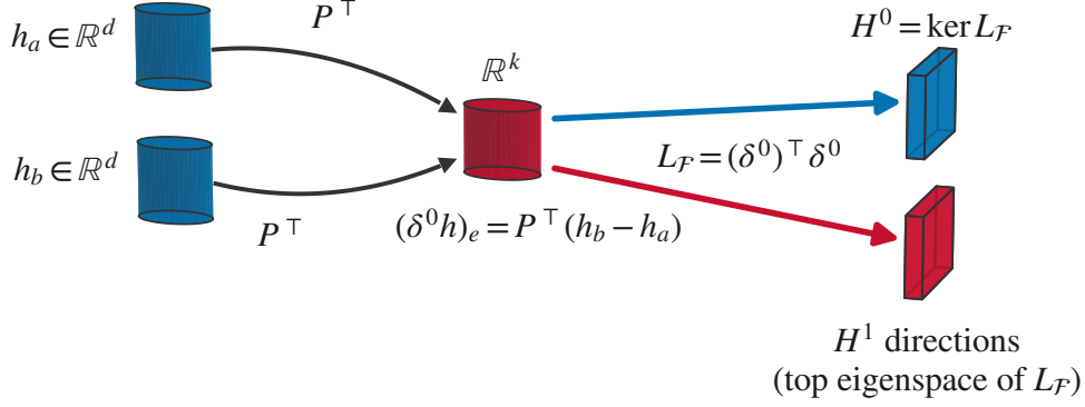
Figure 1: Sheaf decomposition of a paraphrase pair. Hidden states h_a, h_b pass through P^\top into the edge stalk \mathbb{R}^k , where the coboundary measures their disagreement, (\delta^0 h)_e = P^\top(h_b - h_a) . The bottom and top eigenspaces of the sheaf Laplacian L_{\mathcal{F}} split the edge stalk \mathbb{R}^k into H^0 (blue, content stable across phrasing) and the H^1 directions (red, context-dependent variation).
