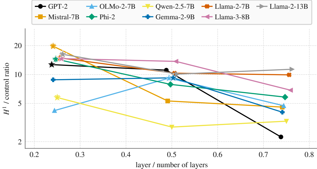
Figure 5: H^1 -to-control effect ratio (protocol b of Table 3) at three depths per architecture, L/4 , L/2 and 3L/4 , plotted against normalized depth (layer index over number of layers). Stars mark each architecture’s largest measured ratio, and points are offset slightly in depth so overlapping peaks stay visible. Only measured points are shown. The GPT-2 and Llama values here come from protocol b and differ from their protocol- a rows in Table 3.
