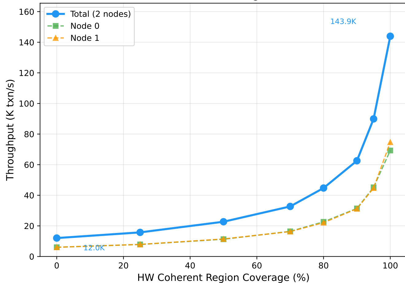
TPC-C New Order Throughput vs. HW Coherent Region Size
