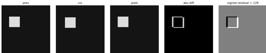
Figure 1: Previous-frame baseline on (t=0, t=1) . From left to right: I_{t-1} , I_t , prediction, |I_t - I_{t-1}| , signed residual + 128. The double-edge structure of the absolute residual is the textbook signature of un-compensated translation.
