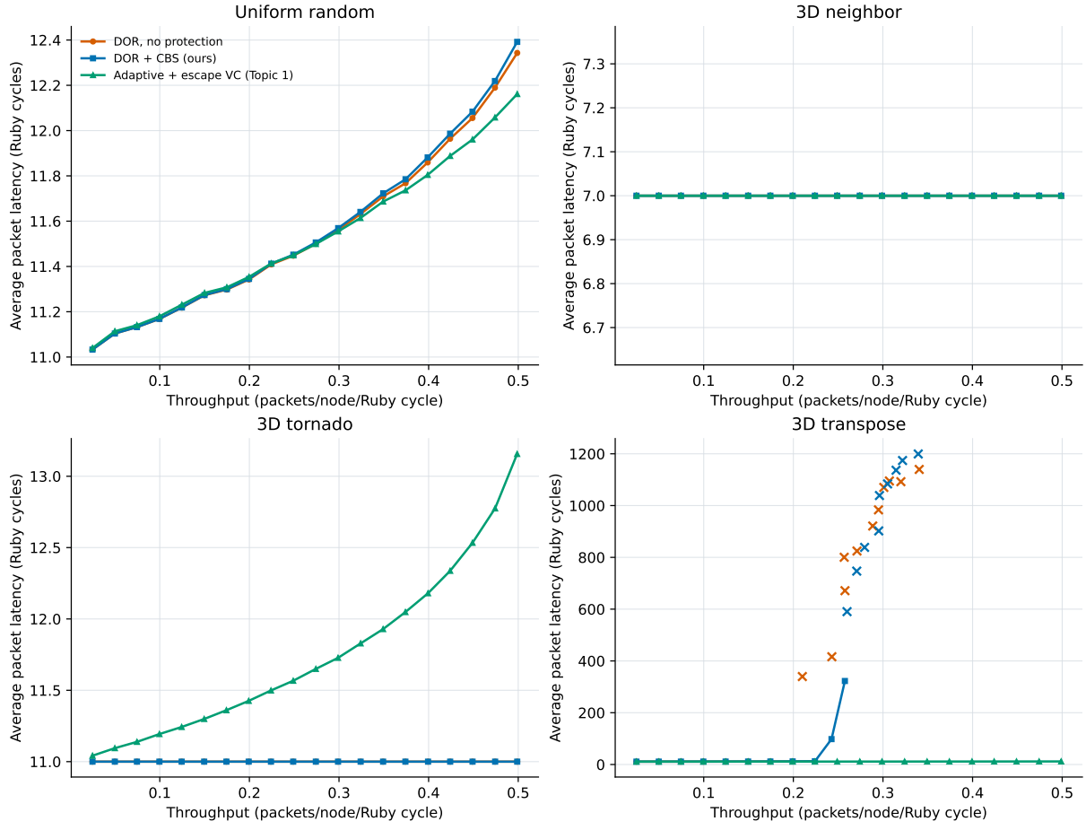
Figure 7: Latency versus offered load for the three modes over the four main traffic patterns. The CBS curve leaves bare DOR only on transpose, where it delays saturation.
