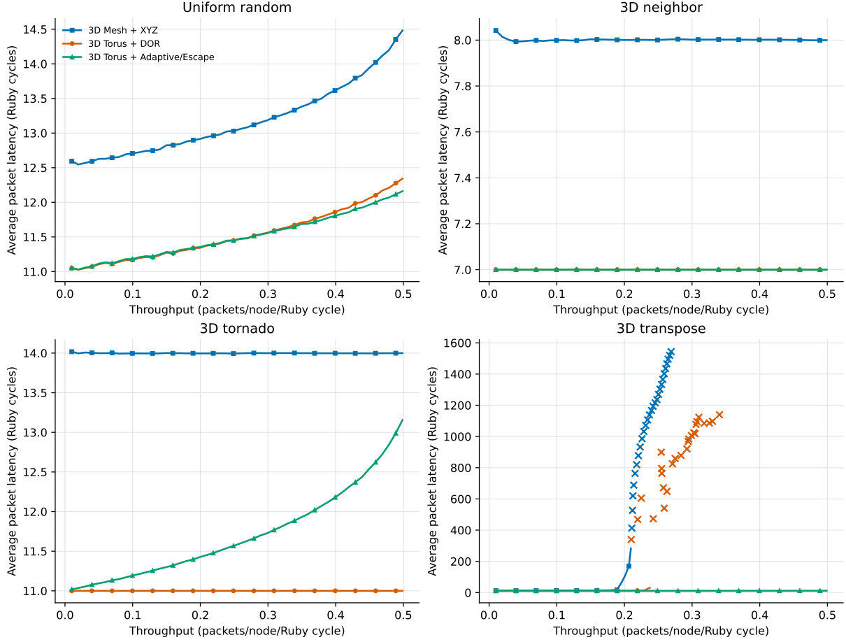
Figure 3: Latency and delivered throughput for the four main traffic patterns.
