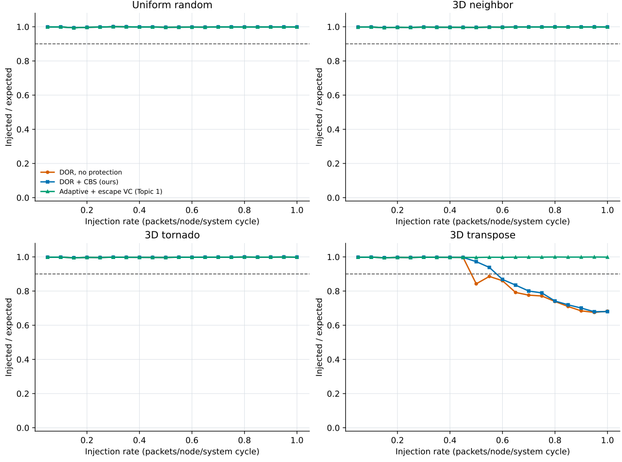
Figure 8: Source acceptance under the CBS sweep. CBS moves the transpose stall point from rate 0.5 to 0.6 and matches bare DOR elsewhere.
