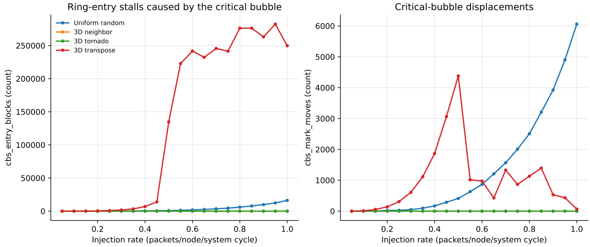
Figure 9: CBS event counters versus injection rate. Entry blocks track congestion depth; mark moves peak at the saturation knee and fall back.
