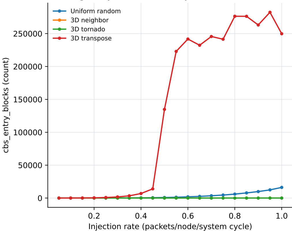
Ring-entry stalls caused by the critical bubble
