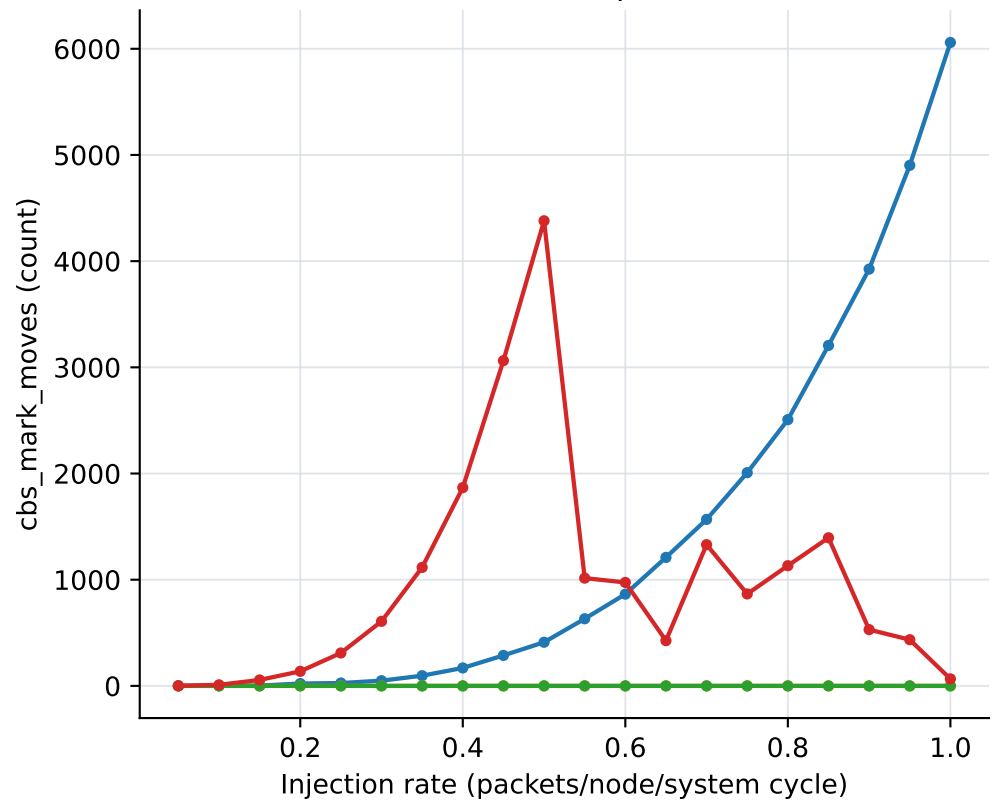
Critical-bubble displacements
