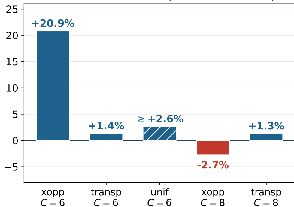
DP-CBS vs. baseline (informative cells)
