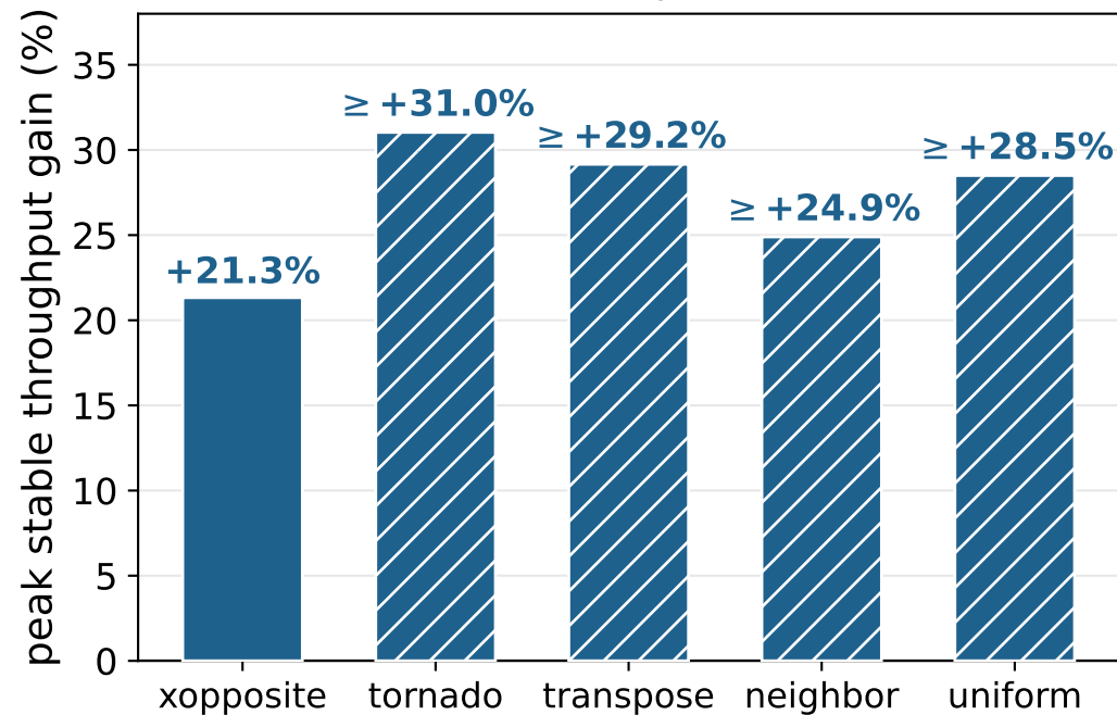
DP-ESC vs. baseline, C = 6 (hatched = lower bound)
