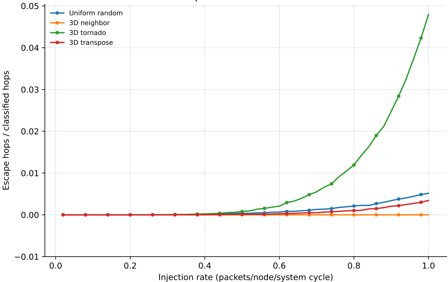
Escape subnetwork utilization
