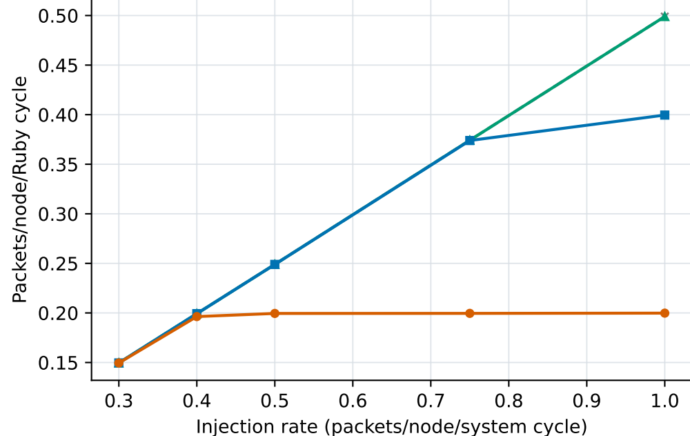
3D X-opposite: throughput
