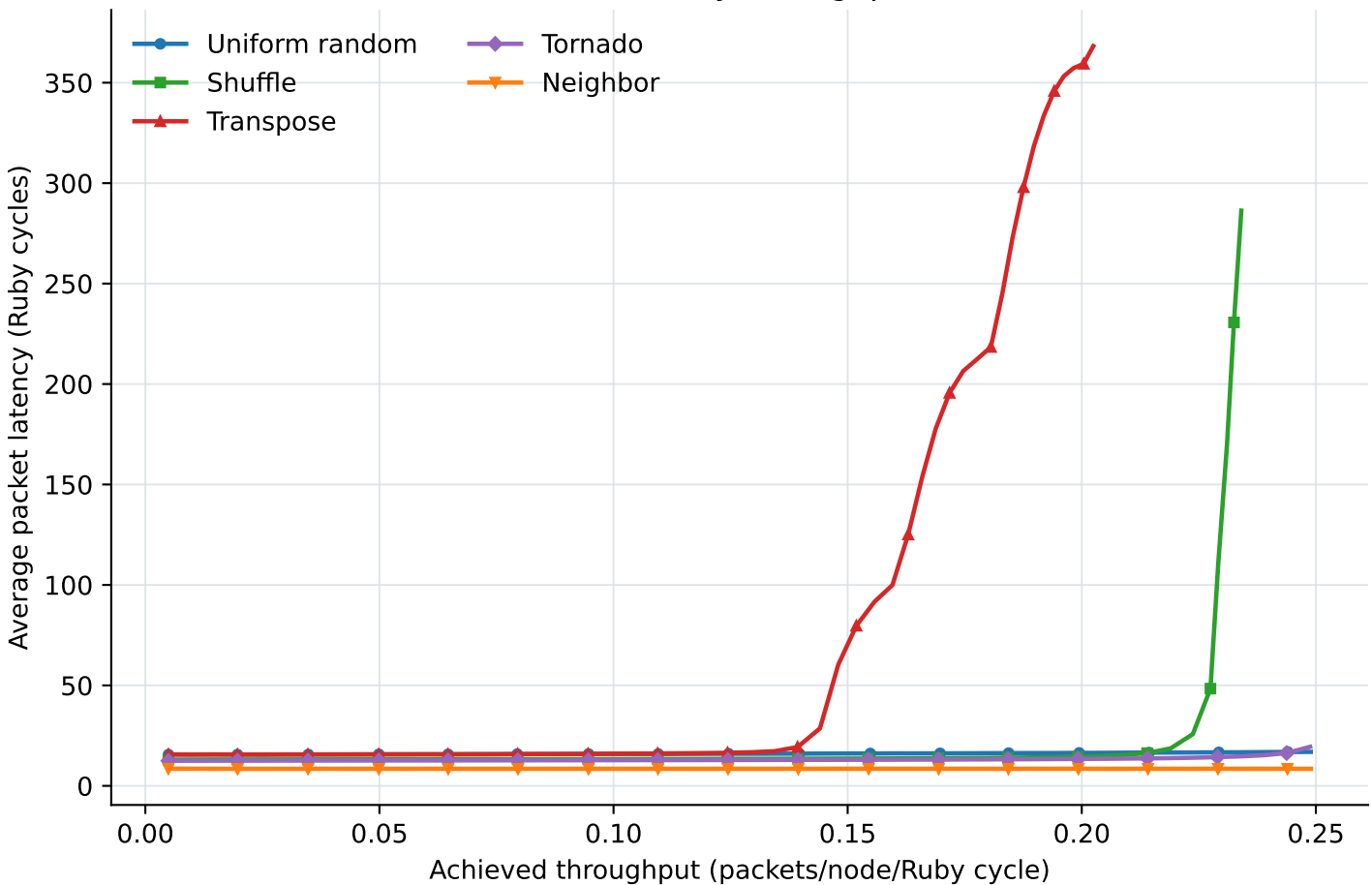
8x8 Mesh: Latency-Throughput Curves
