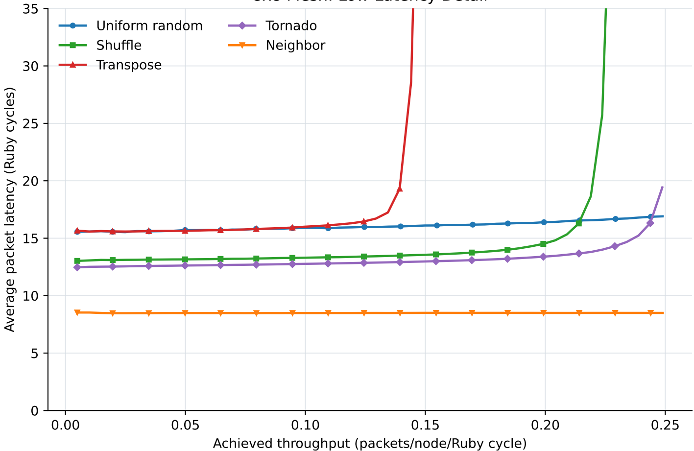
8x8 Mesh: Low-Latency Detail
