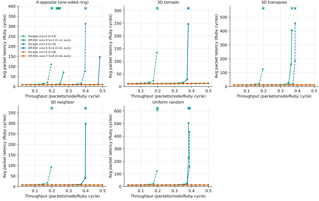
Figure 1: Family B (adaptive + escape): latency–throughput curves per pattern. Solid/dashed lines are stable points; \times markers are unstable points pinned to the top edge. DP curves extend the stable region to higher throughput at equal usable storage.
