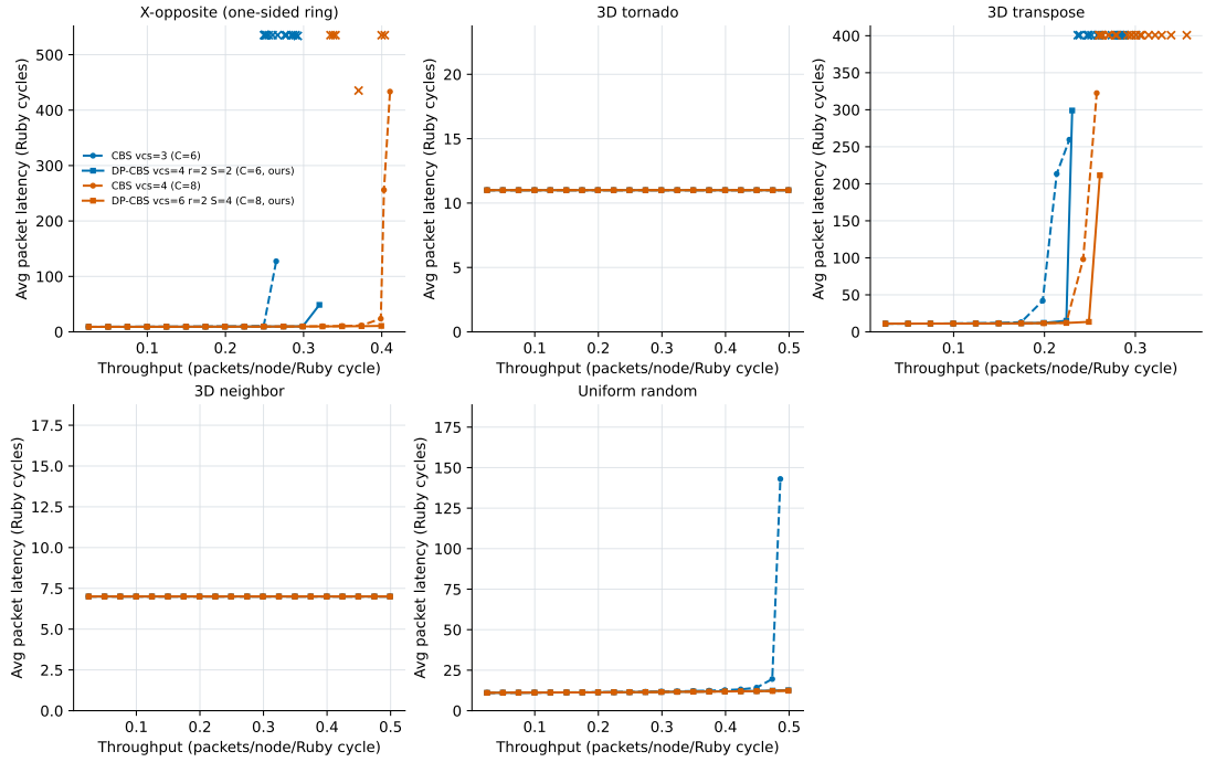
Figure 2: Family A (DOR + CBS): latency–throughput curves per pattern. The xopposite panel shows the +20.9% stable-region extension of A2 over A1; at C=8 (A4 vs. A3) the ordering reverses.
