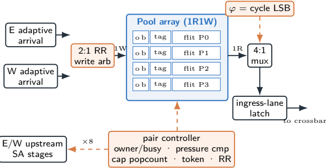
Figure 3: Construction of one pair’s shared bank: a two-request arbiter in front of the single write port, a phase-gated 4:1 read multiplexer onto the winner’s true-ingress crossbar lane, and a local pair controller whose owner/busy bits both upstream allocators observe over a narrow sideband. o, b = per-slot owner and busy bits.
