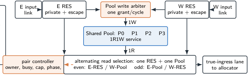
Figure 2: Proposed on-chip organization. (a) Three direction-pair controllers operate in parallel around the normal Garnet switch allocator and crossbar. (b) One pair exposes a single shared Pool read and write service. RES access remains separate; solid arrows are flit/request paths and the sole dashed arrow is controller state. The Pool result is placed on the flit’s true-ingress lane.
