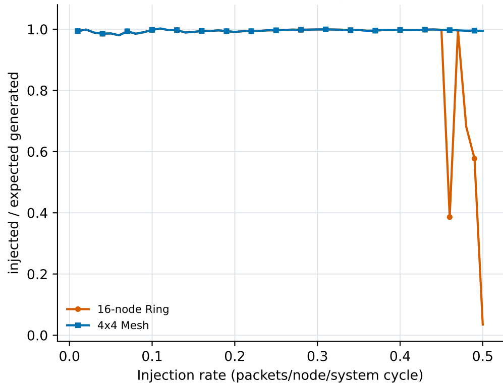
Source injection acceptance
