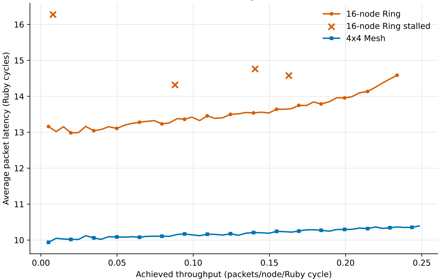
Uniform Random: Ring vs. 4x4 Mesh
