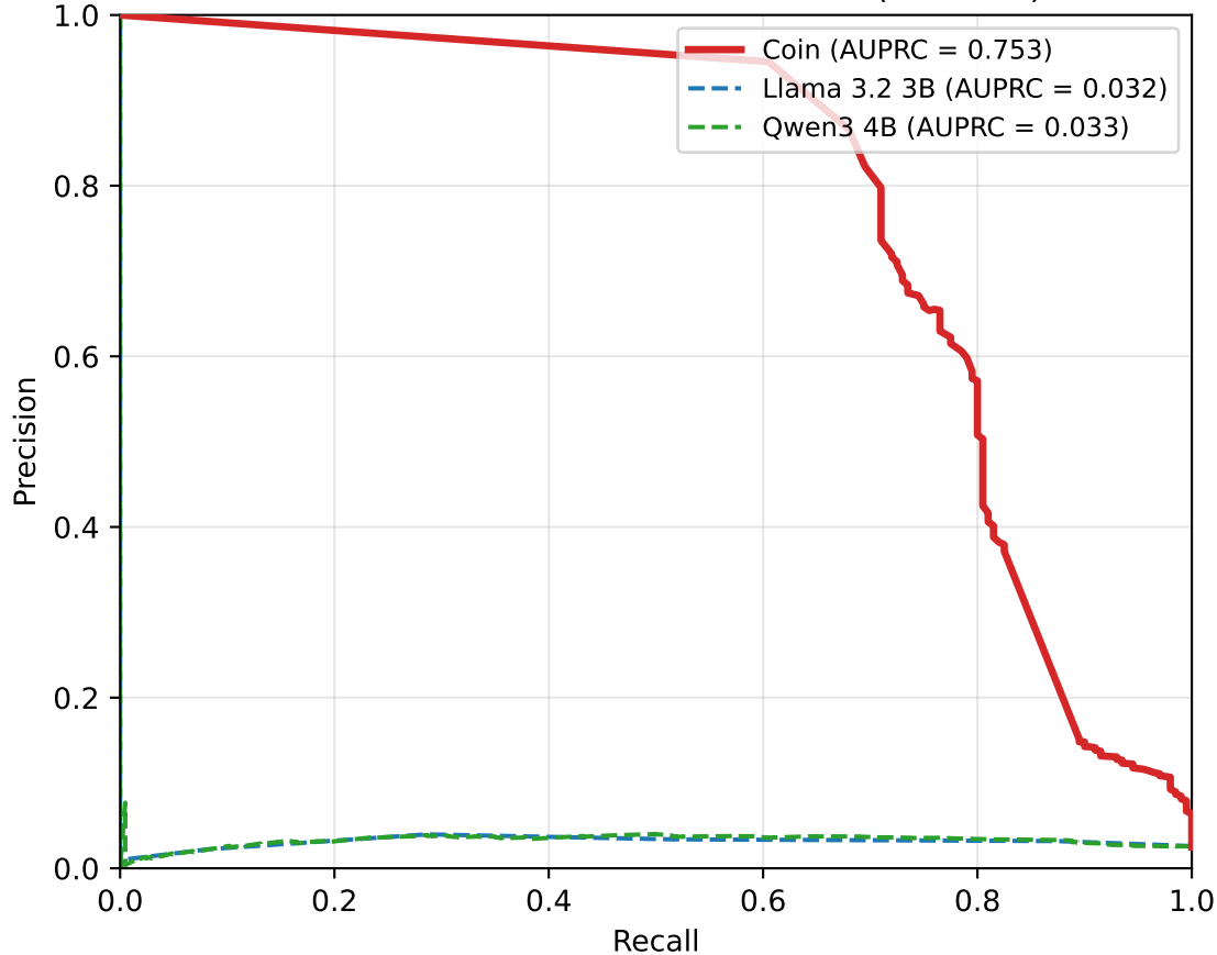
Precision-Recall on MUF detection (n=8000)
