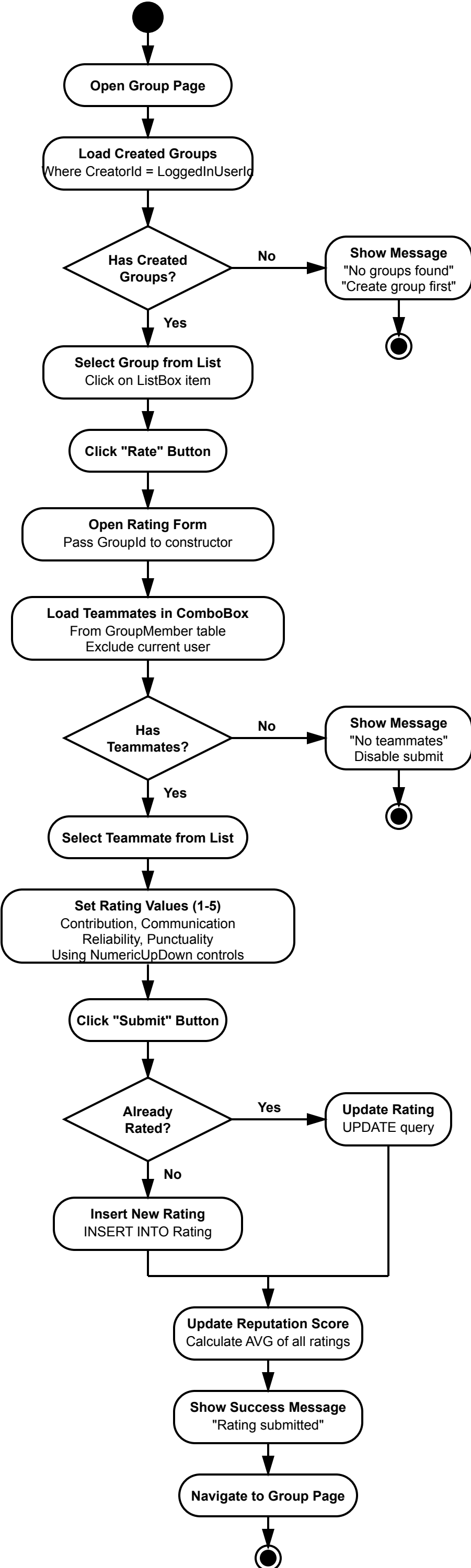
Teammate Rating Activity Diagram
