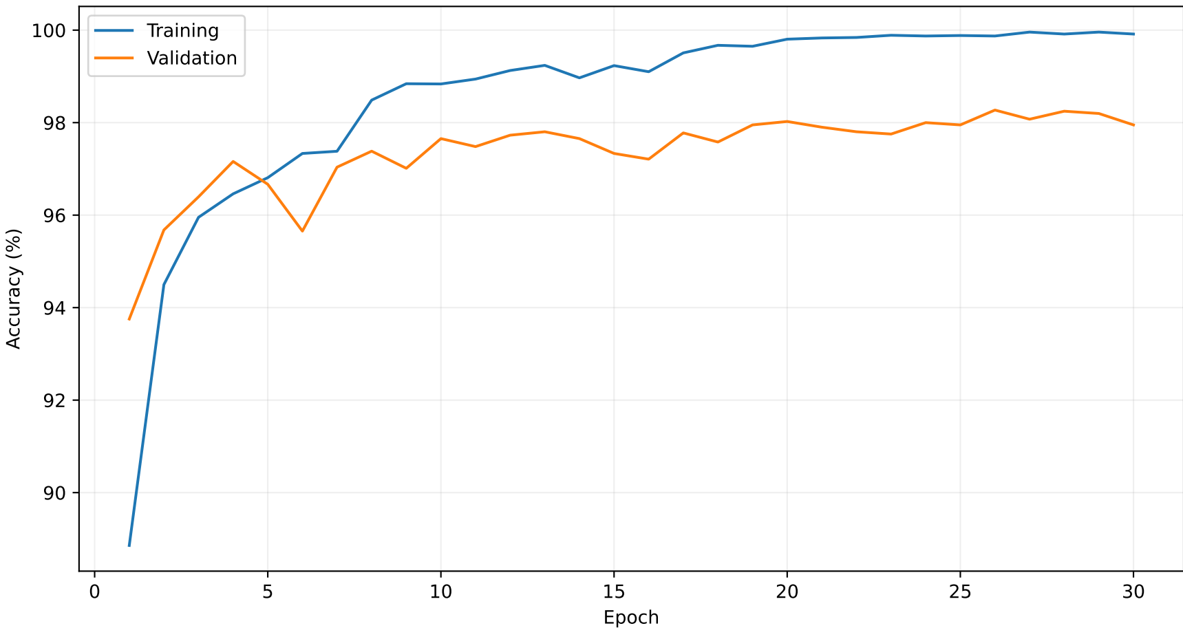
Training vs validation accuracy
