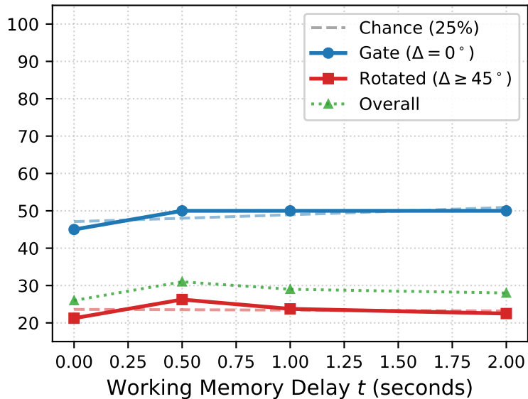
A. Working Memory Decay Trajectory
