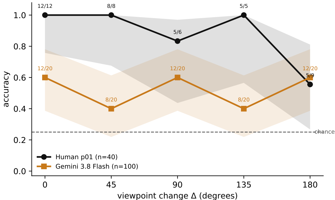
A. Rotation costs the person ( p = 0.047 ). The model shows no effect ( p = 0.65 ).
