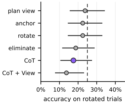
Qwen2.5-VL-32B
