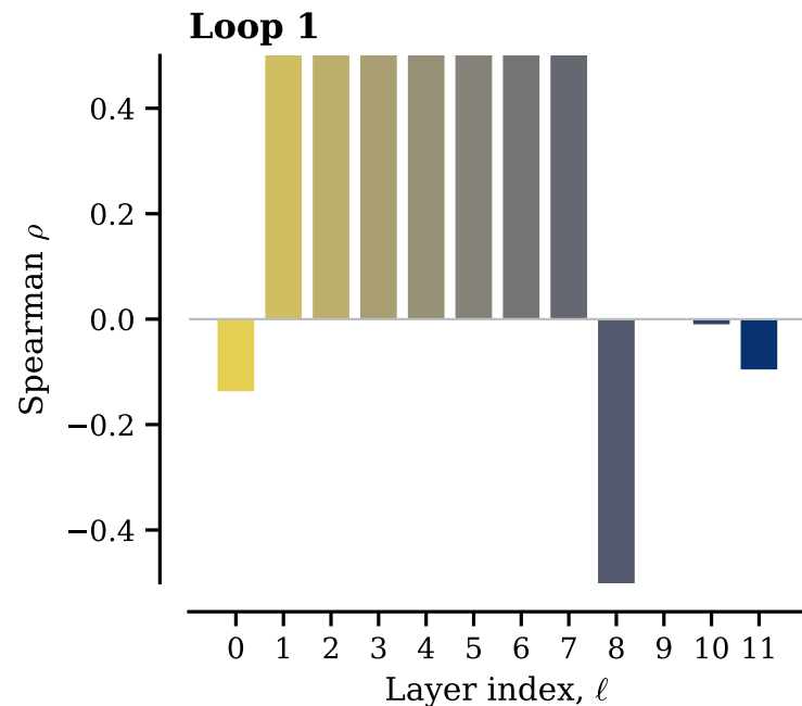
Cos-Sim vs Halt Correlation (after step 5000)
