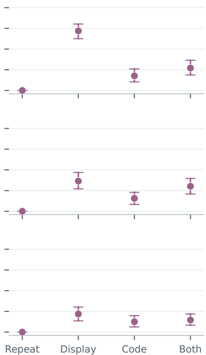
Qwen 8B
