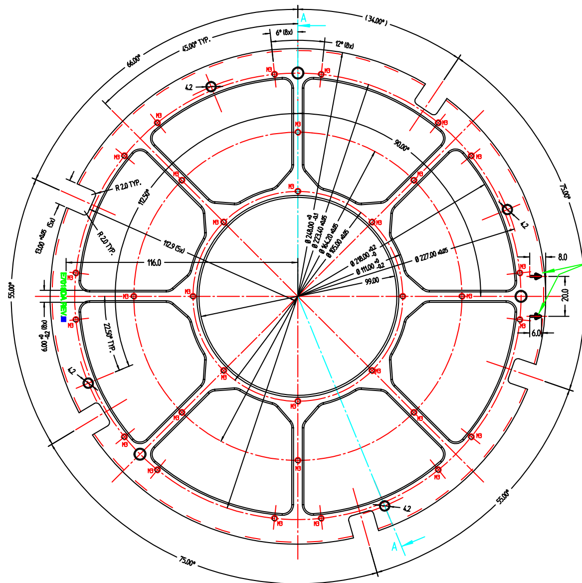
VIEW FROM POGO TOWER SIDE
