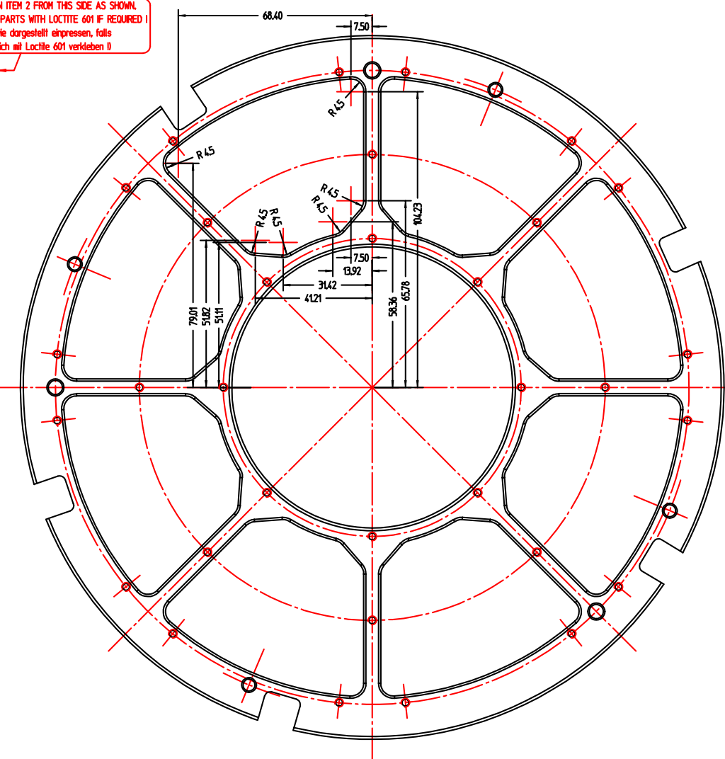
VIEW FROM PROBE CARD SIDE
