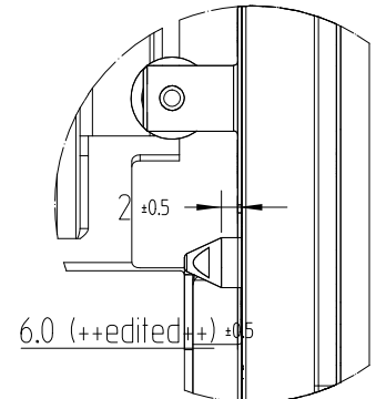
Detail1 Scale 1:1
