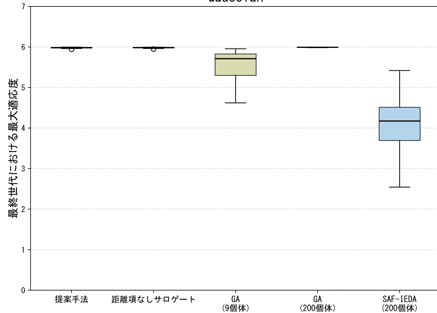
Gaussian_peaks
