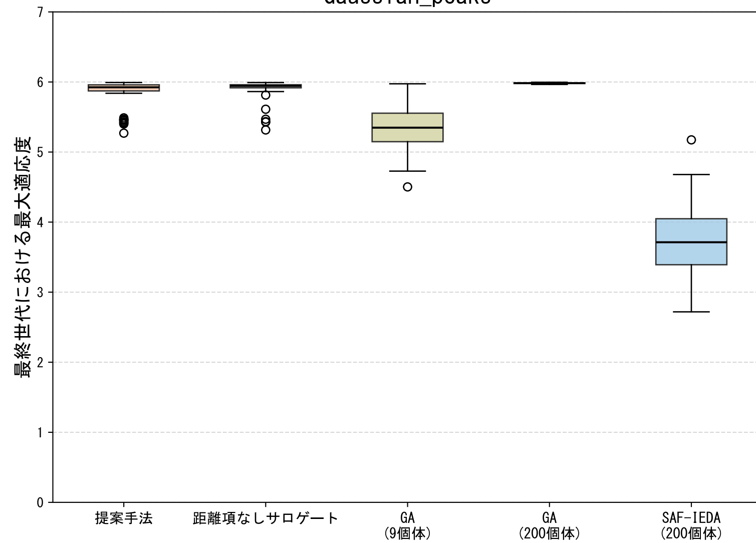
Gaussian_peaks
