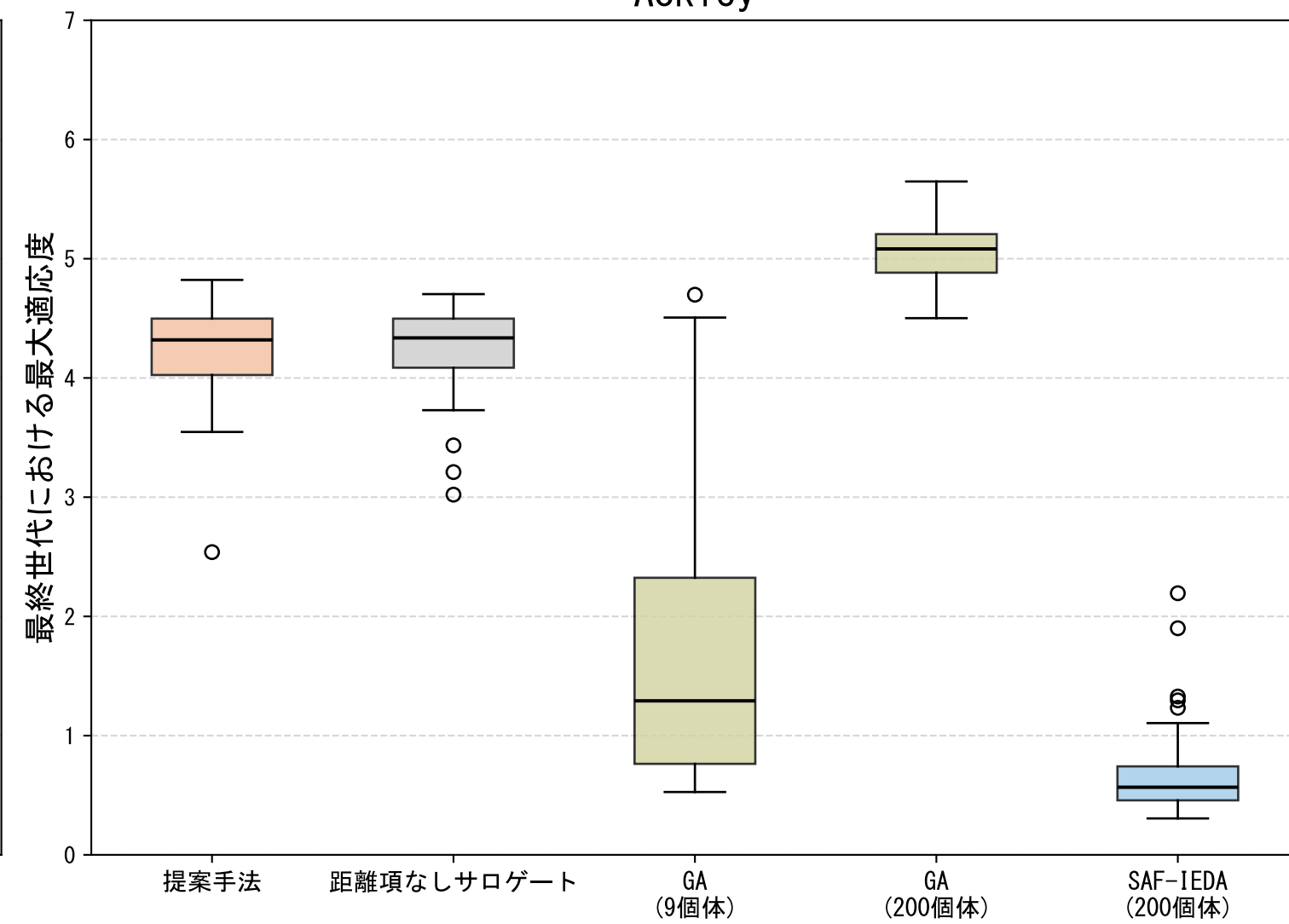
Ackley
