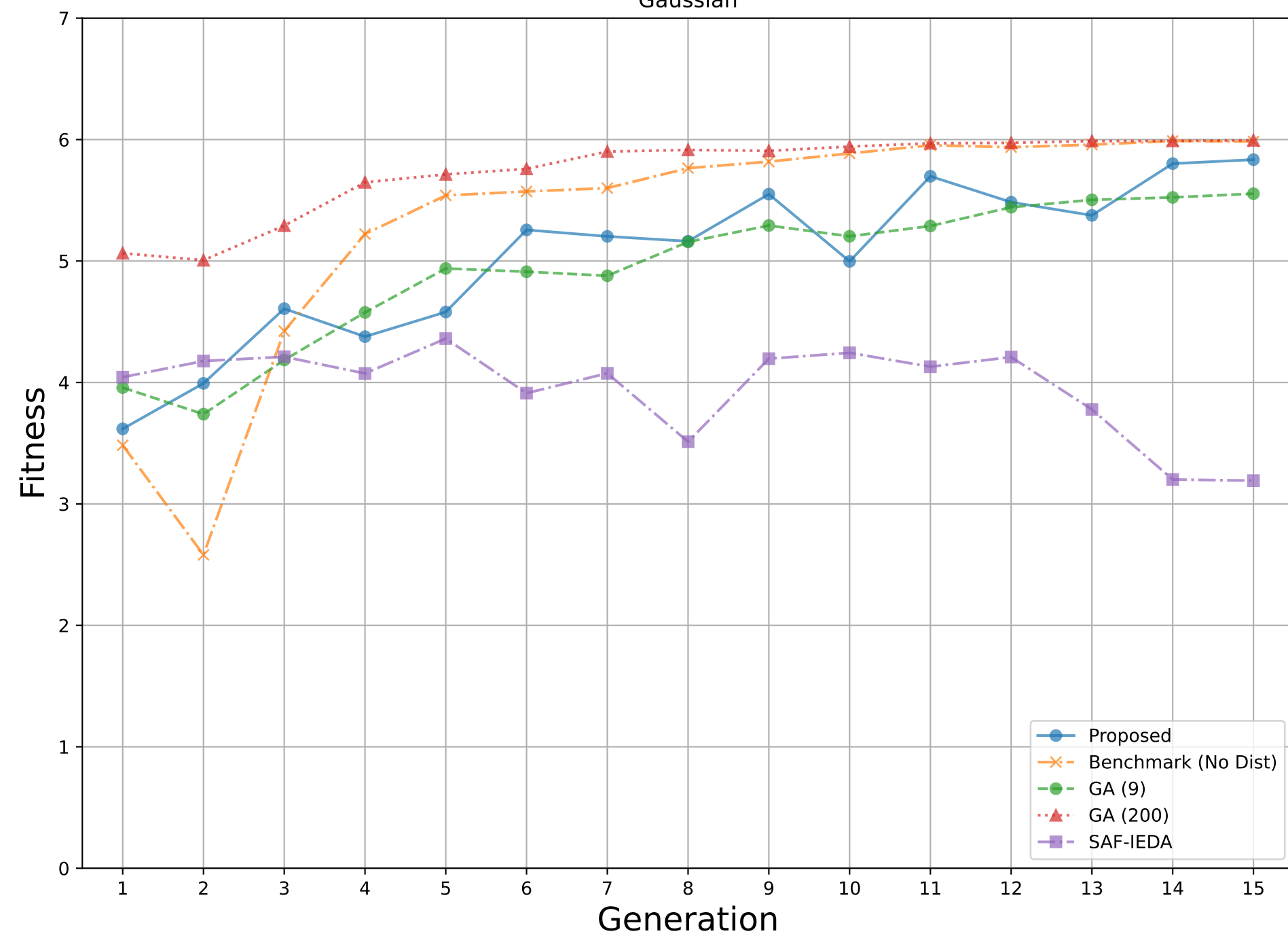
Gaussian_peaks
