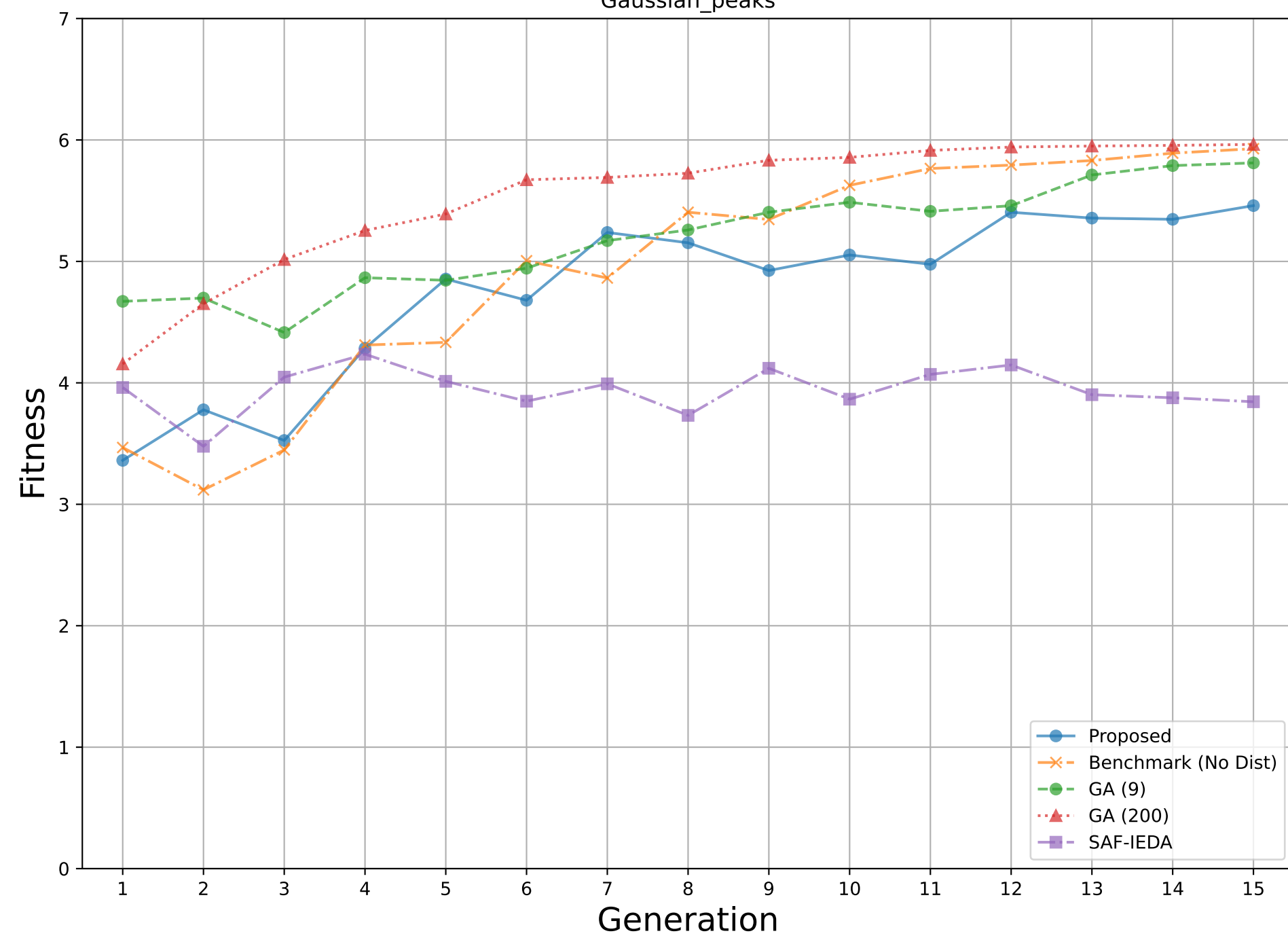
Gaussian_peaks
