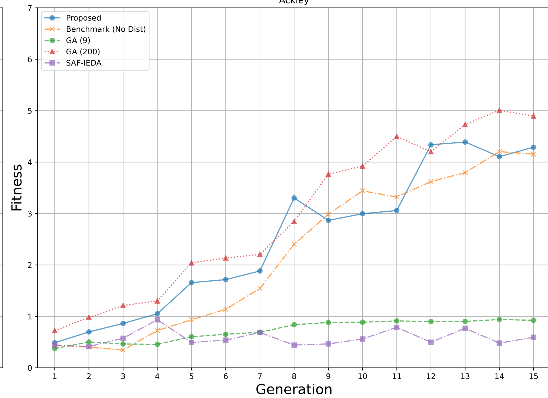
Ackley
