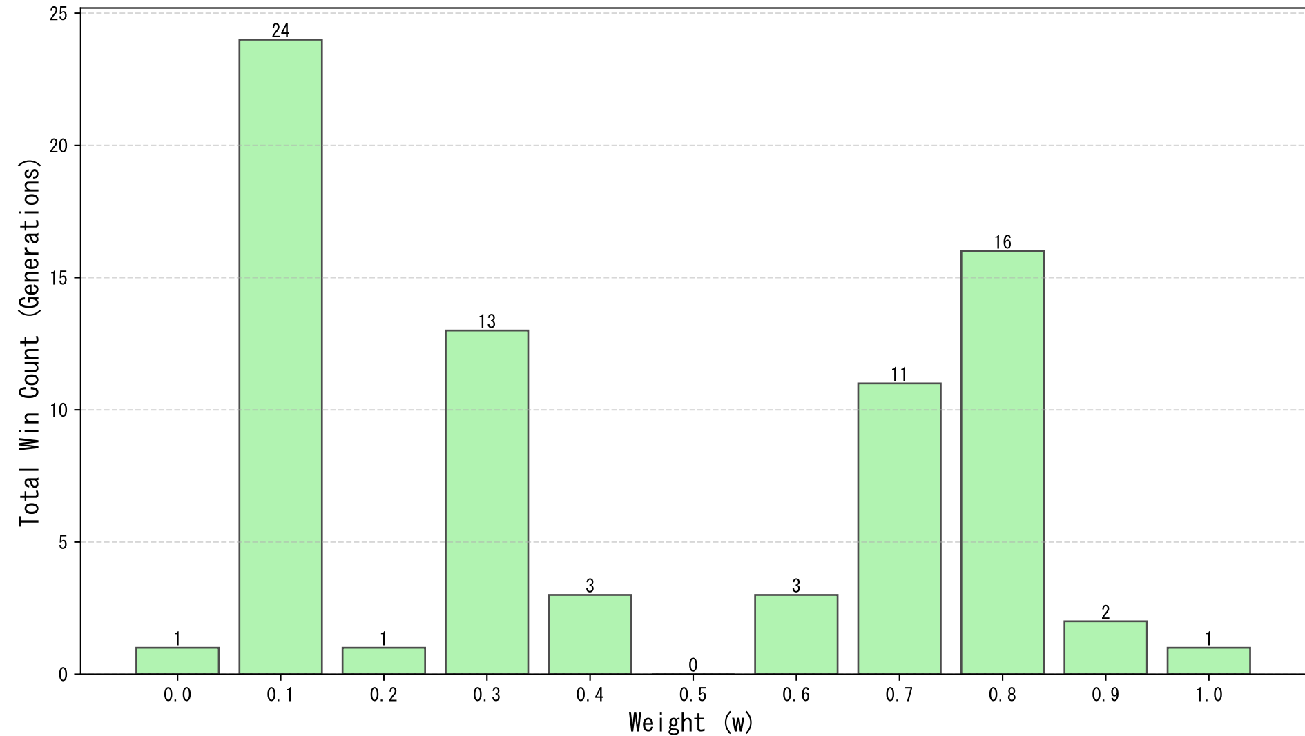
Total Number of Generations with Lowest Avg NN Distance (All Functions)
