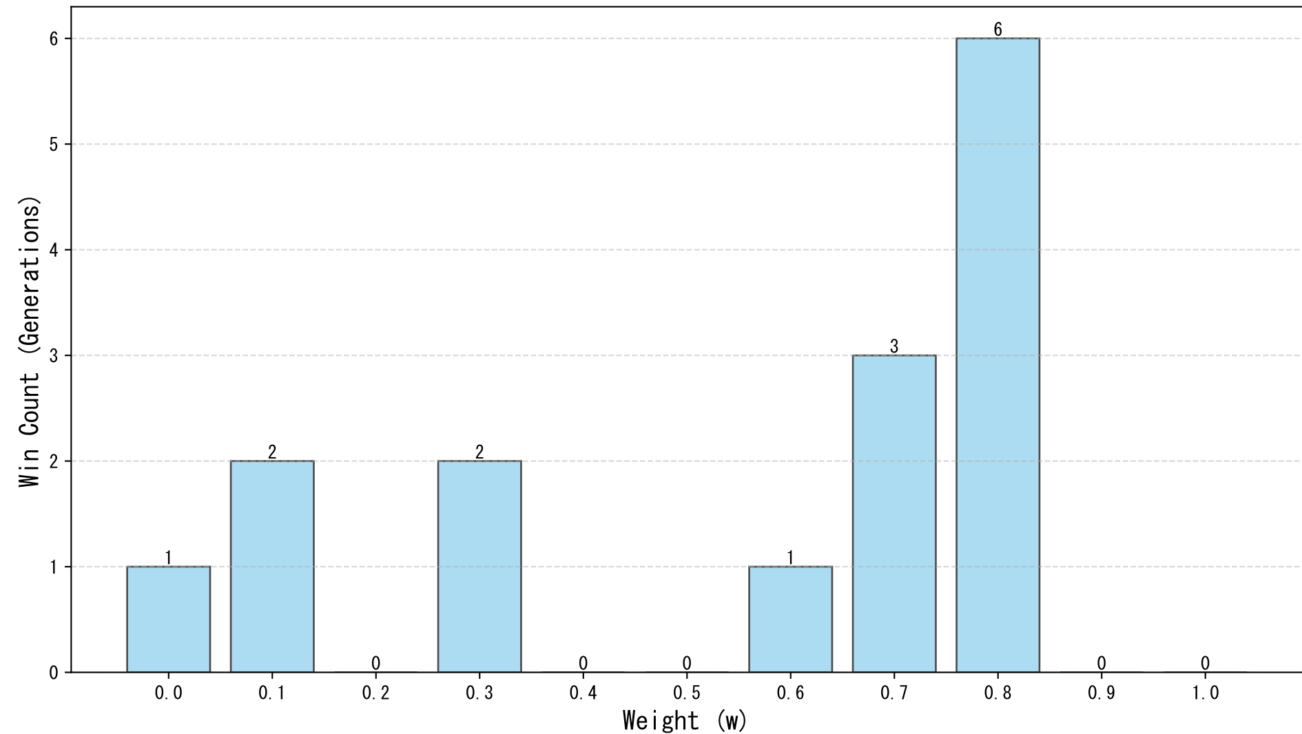
Number of Generations with Lowest Avg NN Distance: Gaussian
