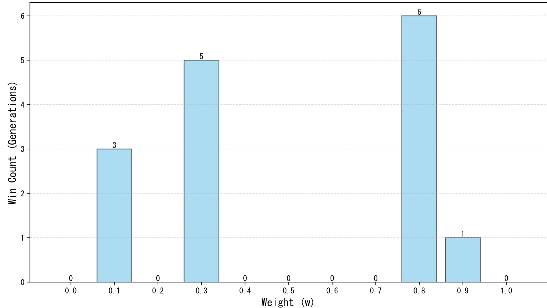
Number of Generations with Lowest Avg NN Distance: Gaussian_cos
