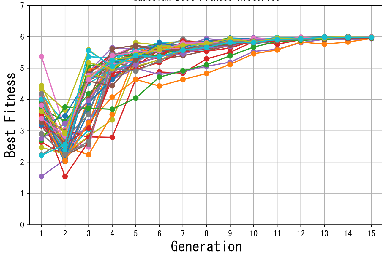
Gaussian Best Fitness Histories
