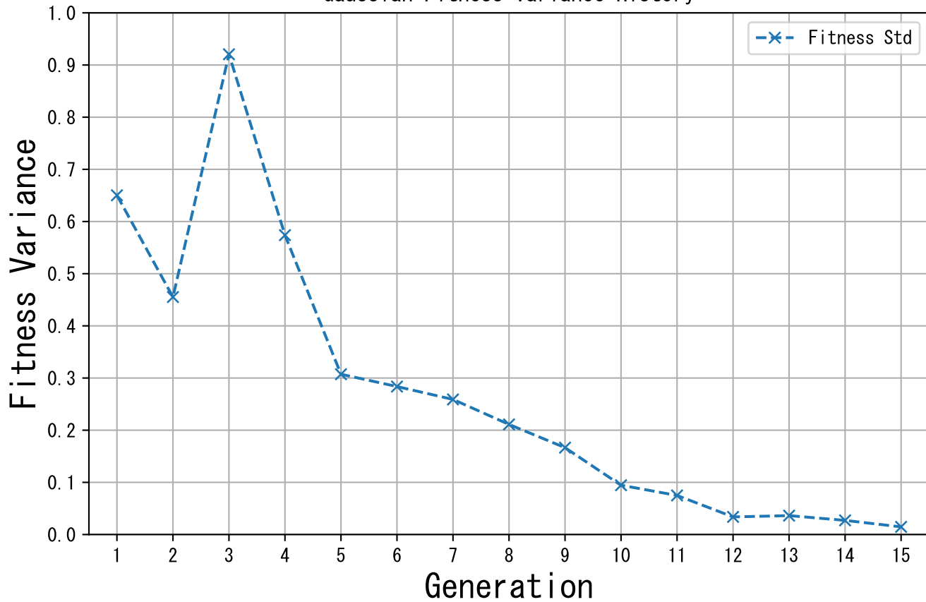
Gaussian Fitness Variance History
