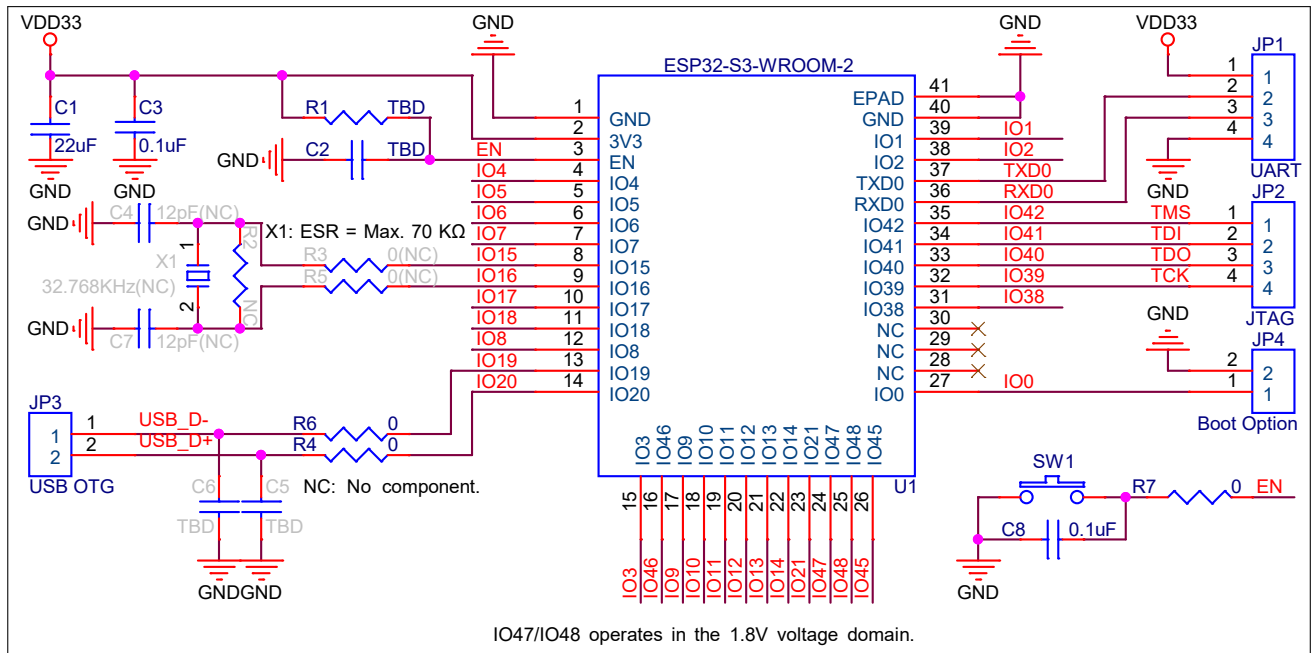
Figure 9-1. Peripheral Schematics
