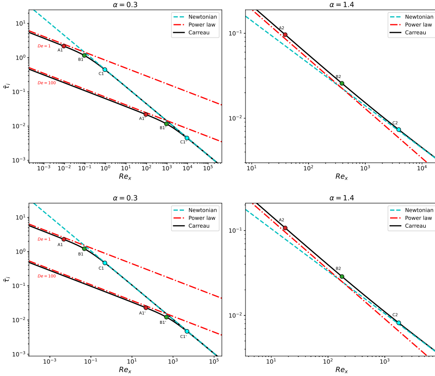
Figure 8. Wall shear for Sakiadis (top) and Blasius (bottom) boundary layers for different power-law exponents \alpha for shear-thinning ( \alpha < 1 ) and shear-thickening ( \alpha > 1 ) regimes at various Deborah numbers De (in the shear-thickening plots, the case De = 100 is shown). The labeled circles denote various Deborah and Reynolds number combinations referred to in Figure 11 to follow.
