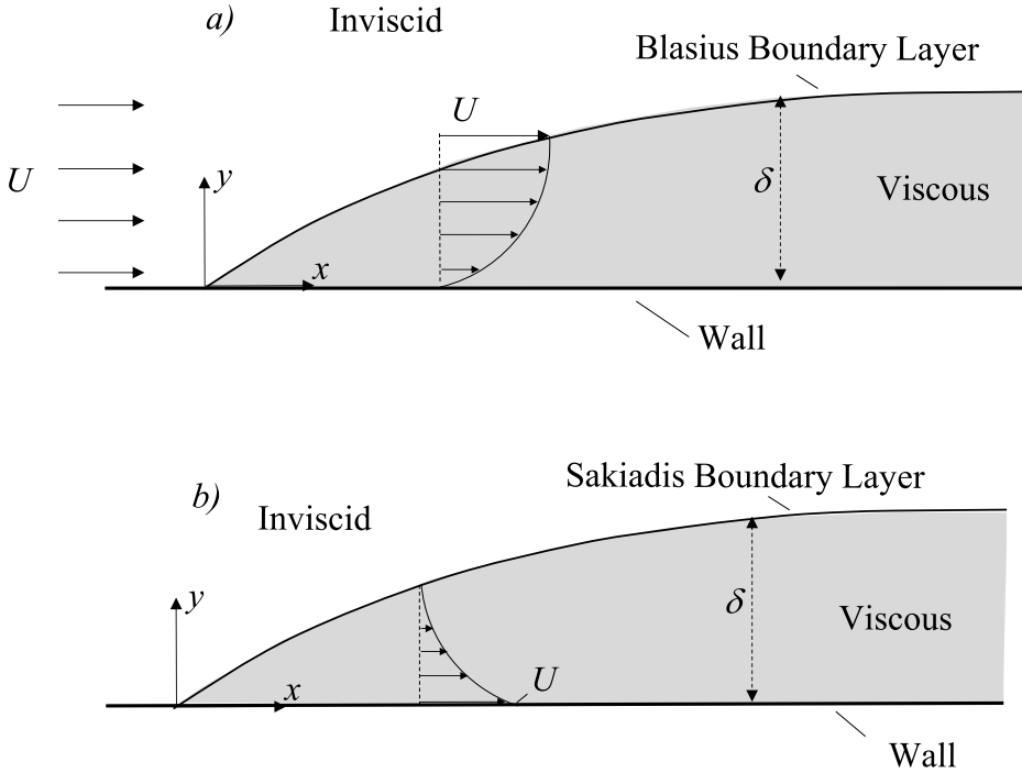
Figure 2. Schematics depicting boundary layer flows along a flat wall. a) Blasius, b) Sakiadis. Here, U is the velocity of the oncoming fluid or wall and \delta is the boundary layer thickness that increases with distance downstream, x .
