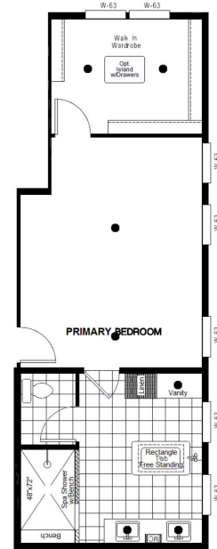
Opt. Glamour Bath #2 / Super Wardrobe
