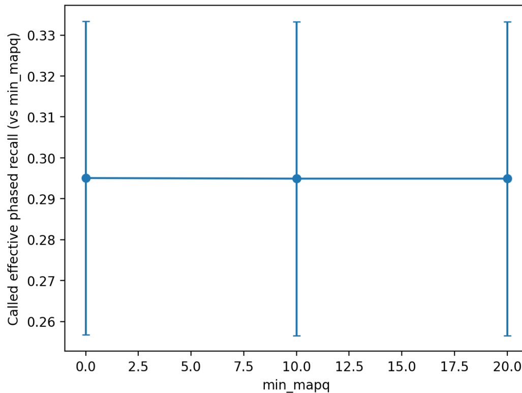
Figure 10.5.2.5 — Called Effective Phased Recall Across the phasing-threshold grid.
