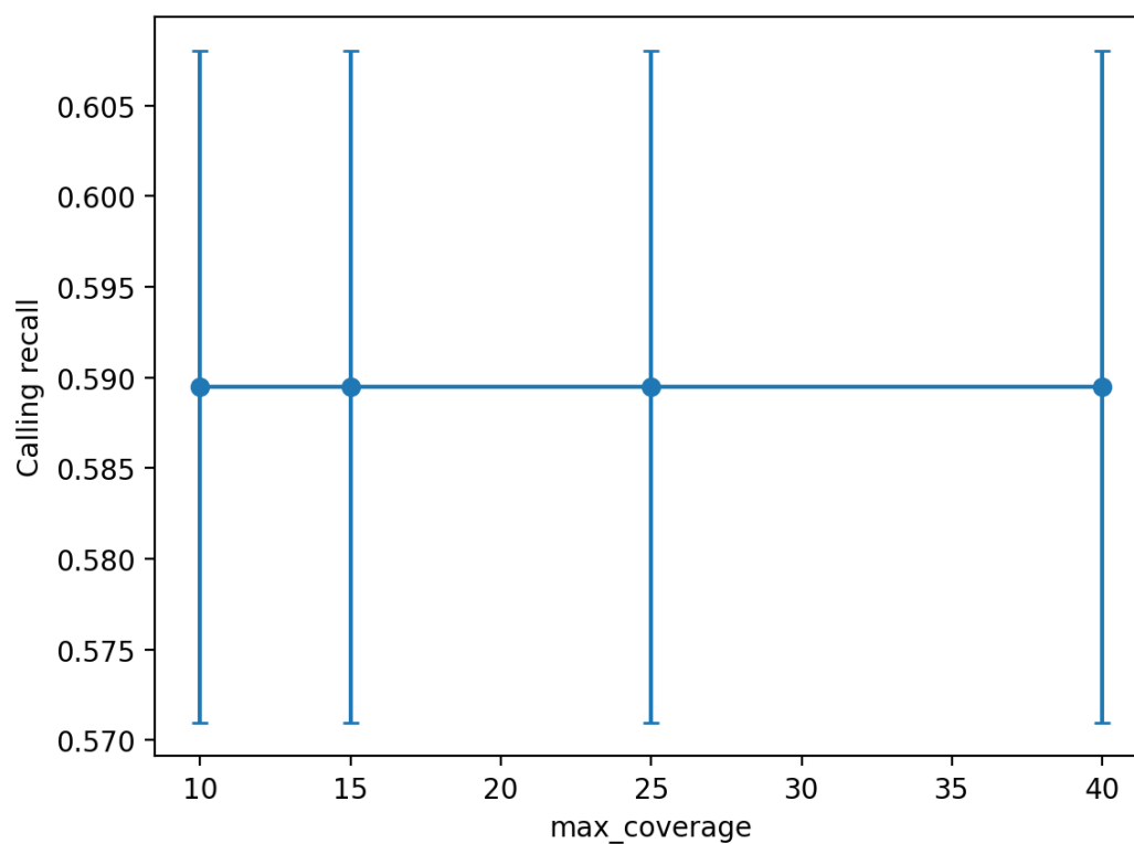
Figure 10.5.2.4 — Variant Calling Recall Rate vs max_coverage.
