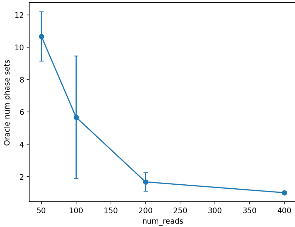
Figure 10.2.4 — Oracle Number of Phase Sets vs num_reads .
