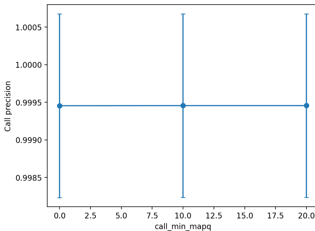
Figure 10.5.2.28 — Variant Calling Precision vs call_min_mapq .
