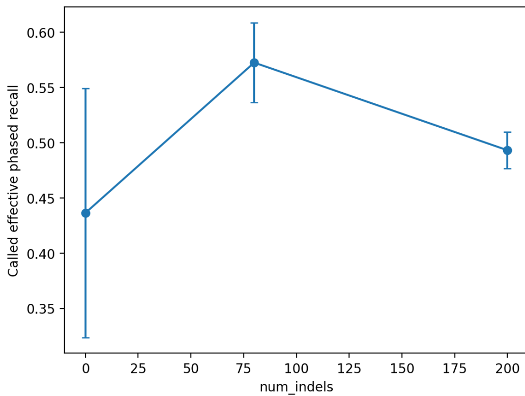
Figure 10.3.5.2 — Called Effective Phased Recall vs num_indels.
