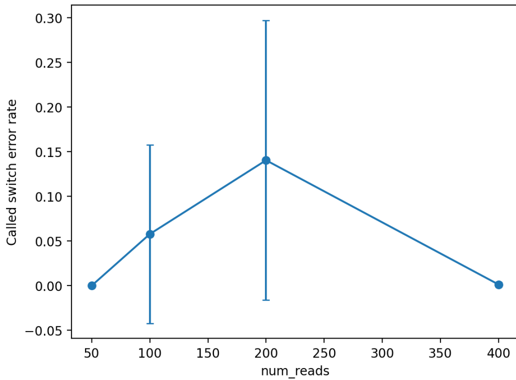
Figure 10.2.6 — Called Switch Error Rate vs num_reads .
