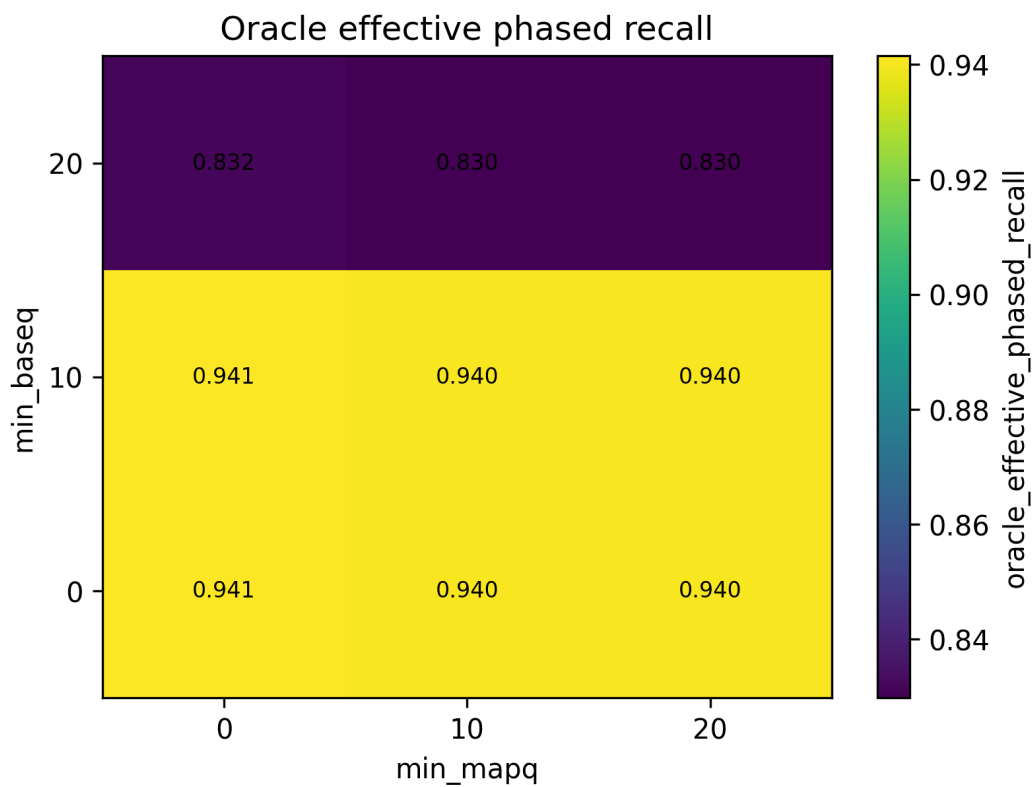
Figure 10.5.2.8 — Oracle Effective Phased Recall Across the phasing-threshold grid (heatmap).
