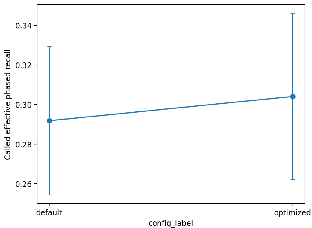
Figure 10.5.3.5 — Called Effective Phased Recall Across representative configurations.
