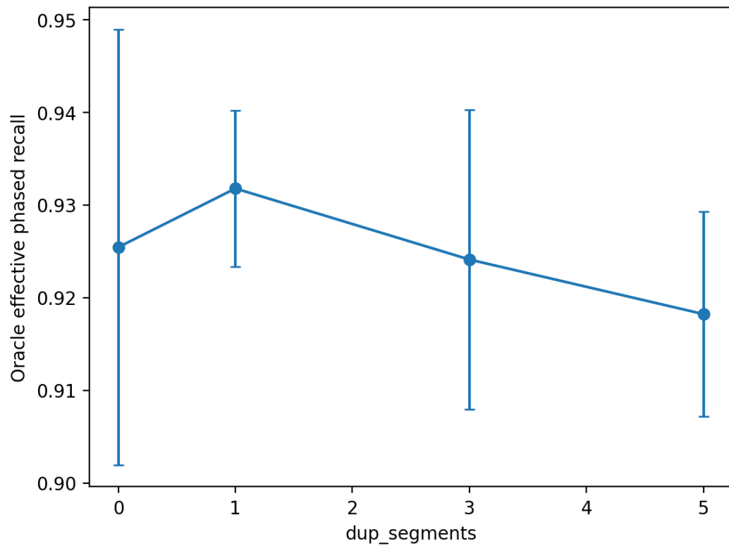
Figure 10.3.1.4 — Oracle Effective Phased Recall vs dup_segments.
