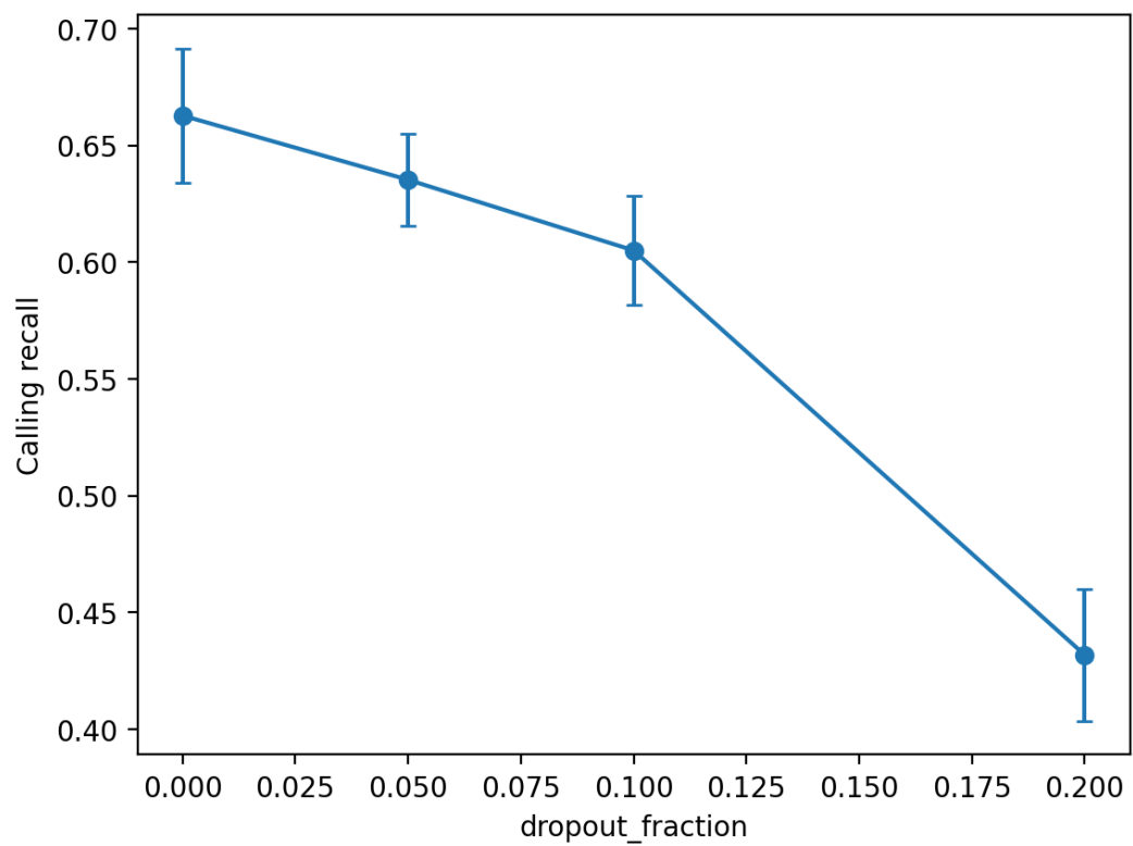
Figure 10.3.2.5 — Variant Calling Recall Rate vs dropout_fraction.
