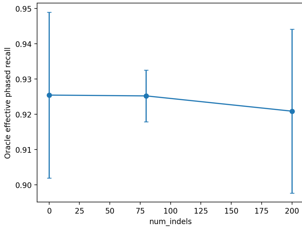
Figure 10.3.5.1 — Oracle Effective Phased Recall vs num_indels.
