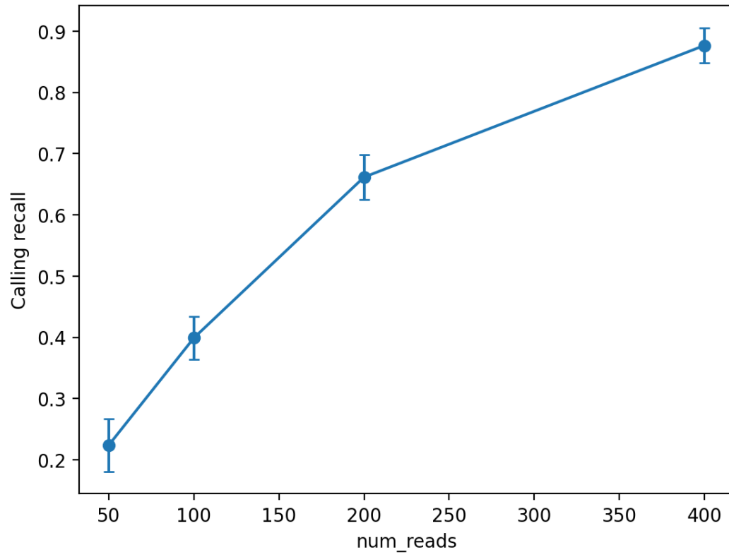
Figure 10.2.1 — Variant Calling Recall Rate vs num_reads.
