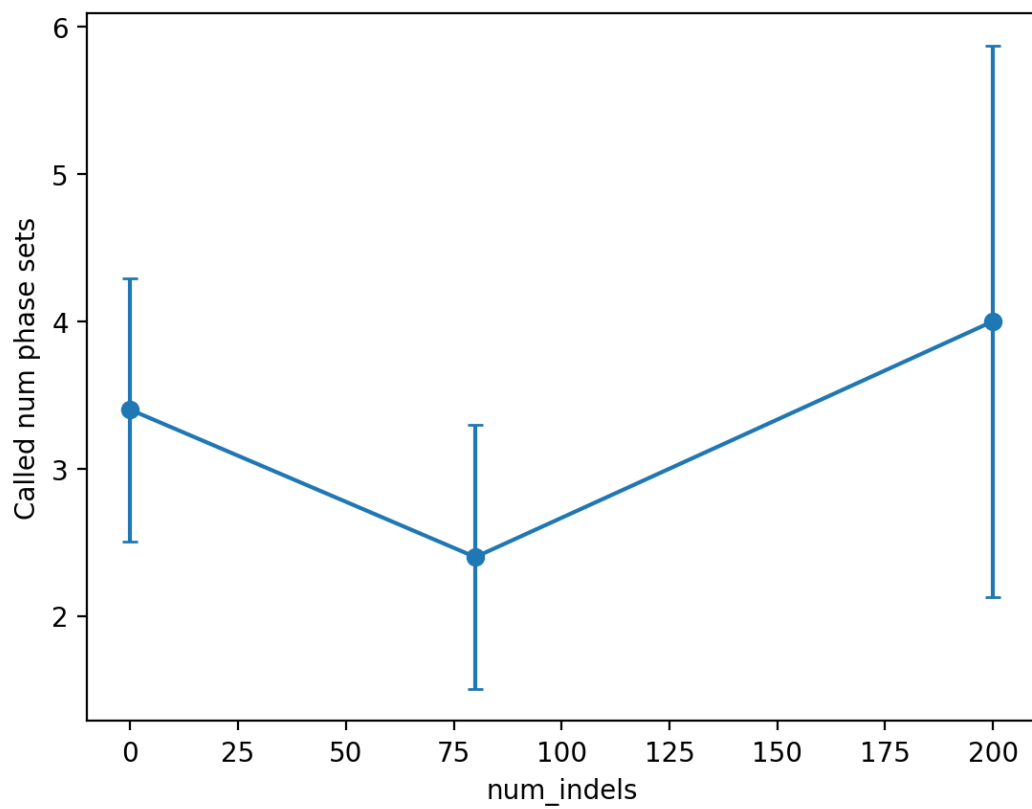
Figure 10.3.5.4 — Called Number of Phase Sets vs num_indels .
