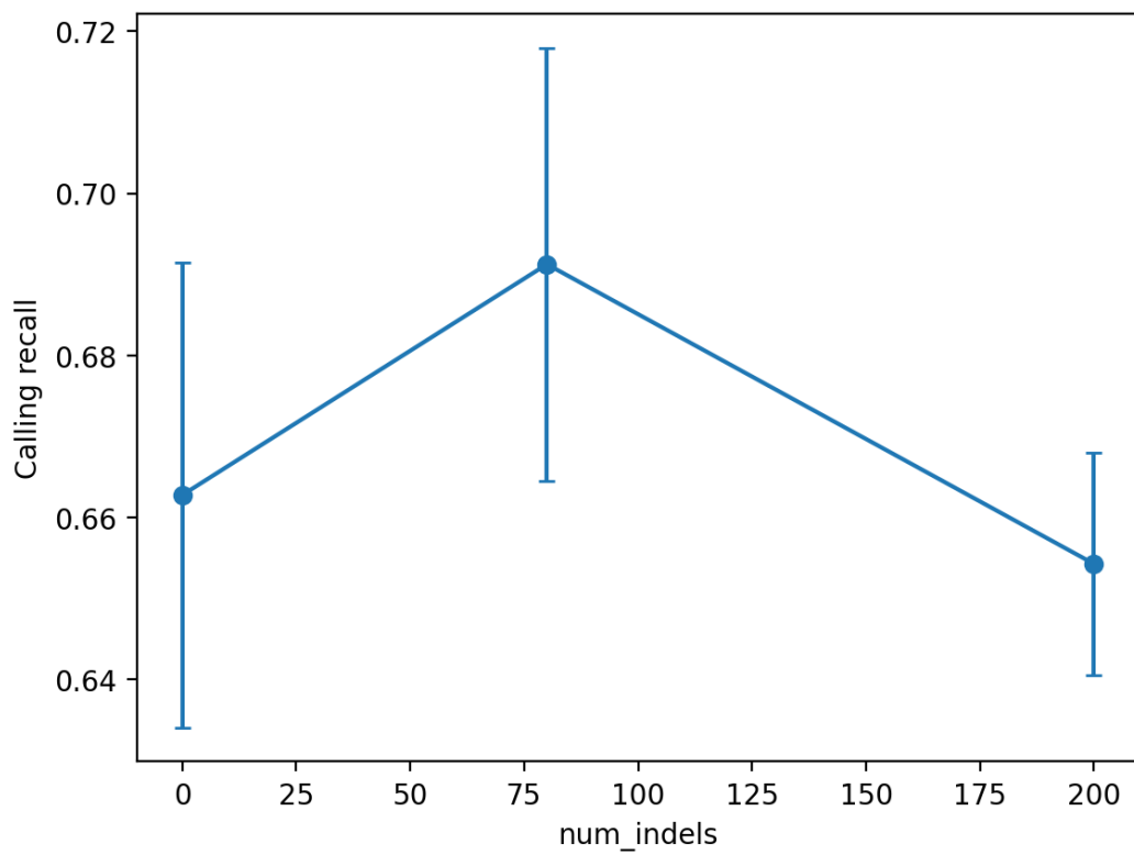
Figure 10.3.5.3 — Variant Calling Recall Rate vs num_indels .
