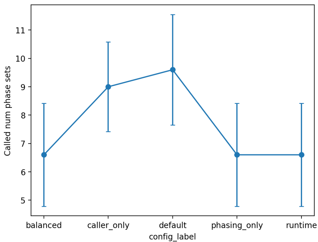
Figure 10.5.3.3 — Called Number of Phase Sets Across representative configurations.
