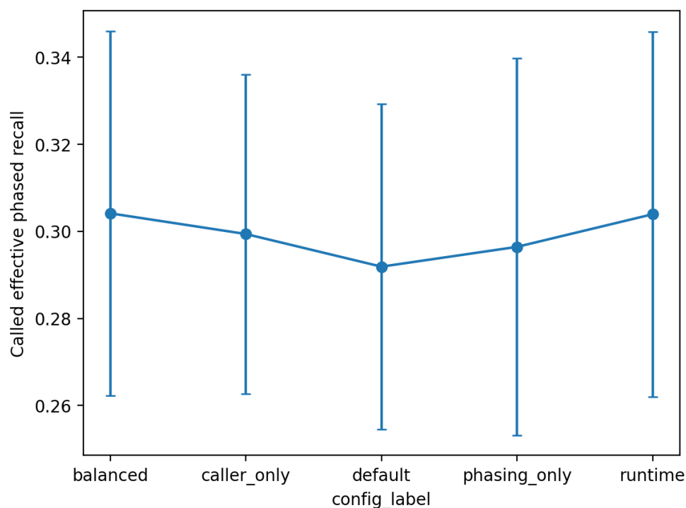
Figure 10.5.3.1 — Called effective phased recall across representative configurations. The optimzied configuration achieves the highest end-to-end phased recall, while the runtime-biased configuration performs almost identically. This shows that combining caller-side and phasing-side tuning yields the strongest practical performance.
