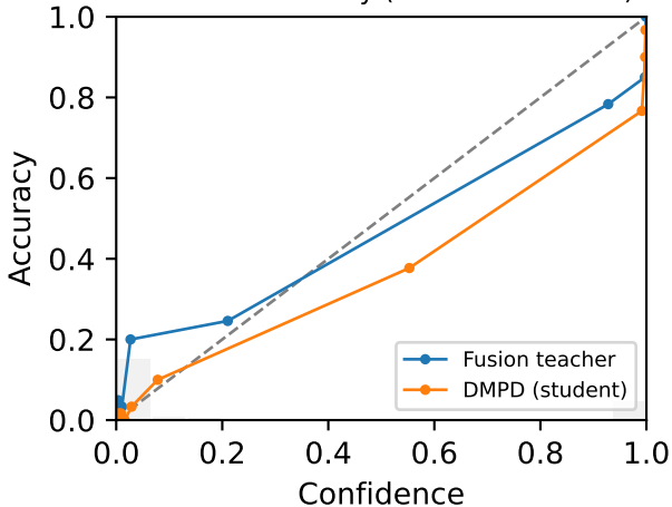
WeFEND reliability (teacher vs DMPD)
