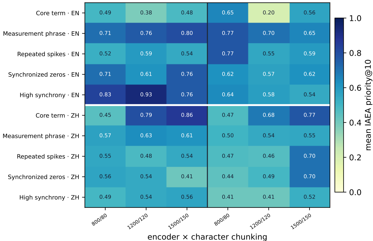
MiniLM-L12
