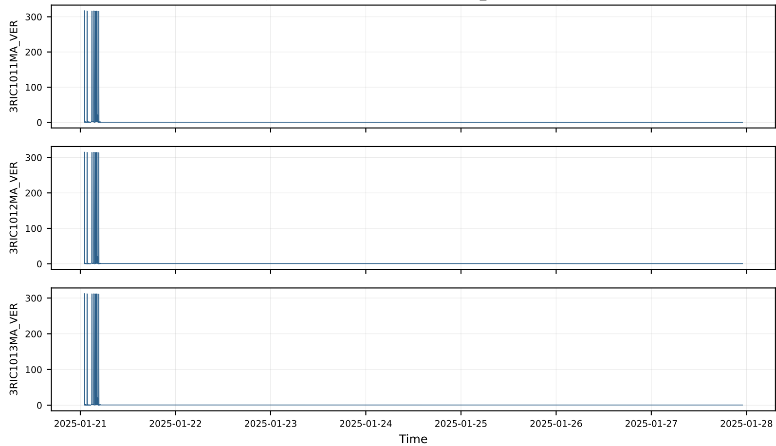
Example neutron-current channels (A1_1, downsampled)
