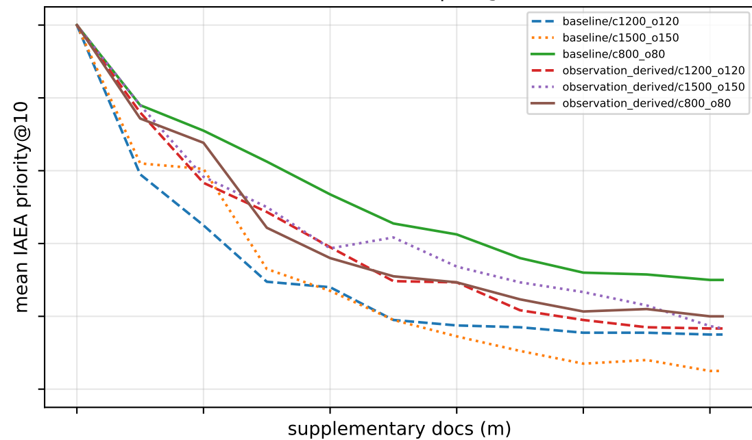
multi-MiniLM-L12-v2 | lang=en
