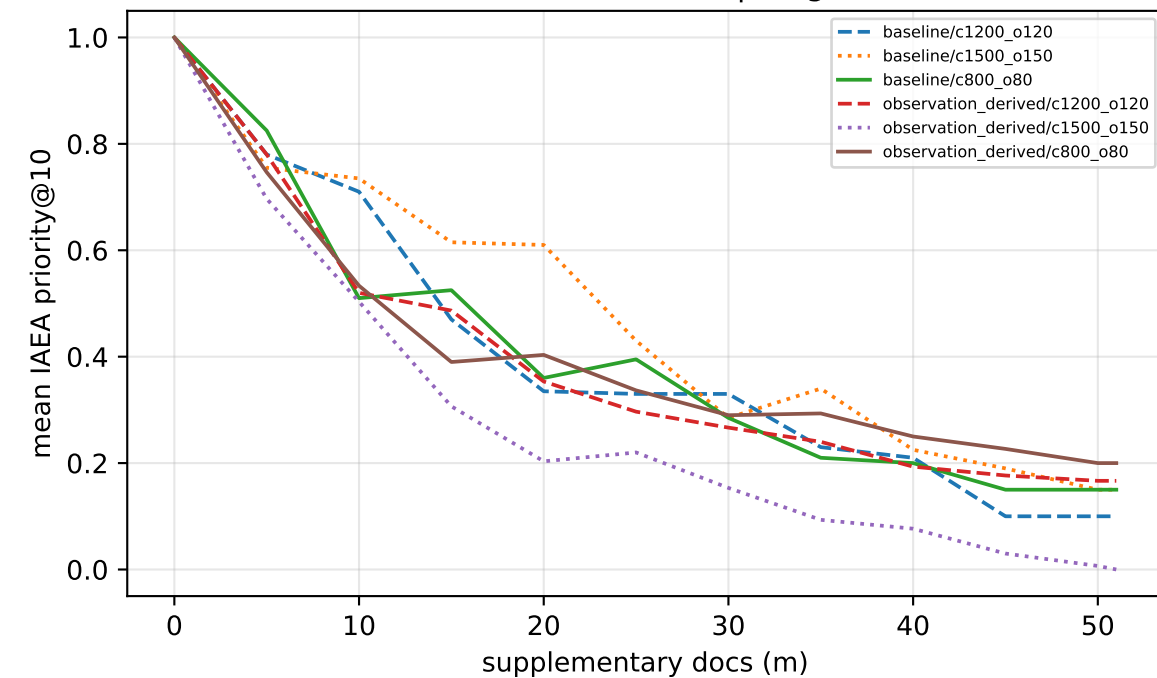
multi-MiniLM-L12-v2 | lang=zh
