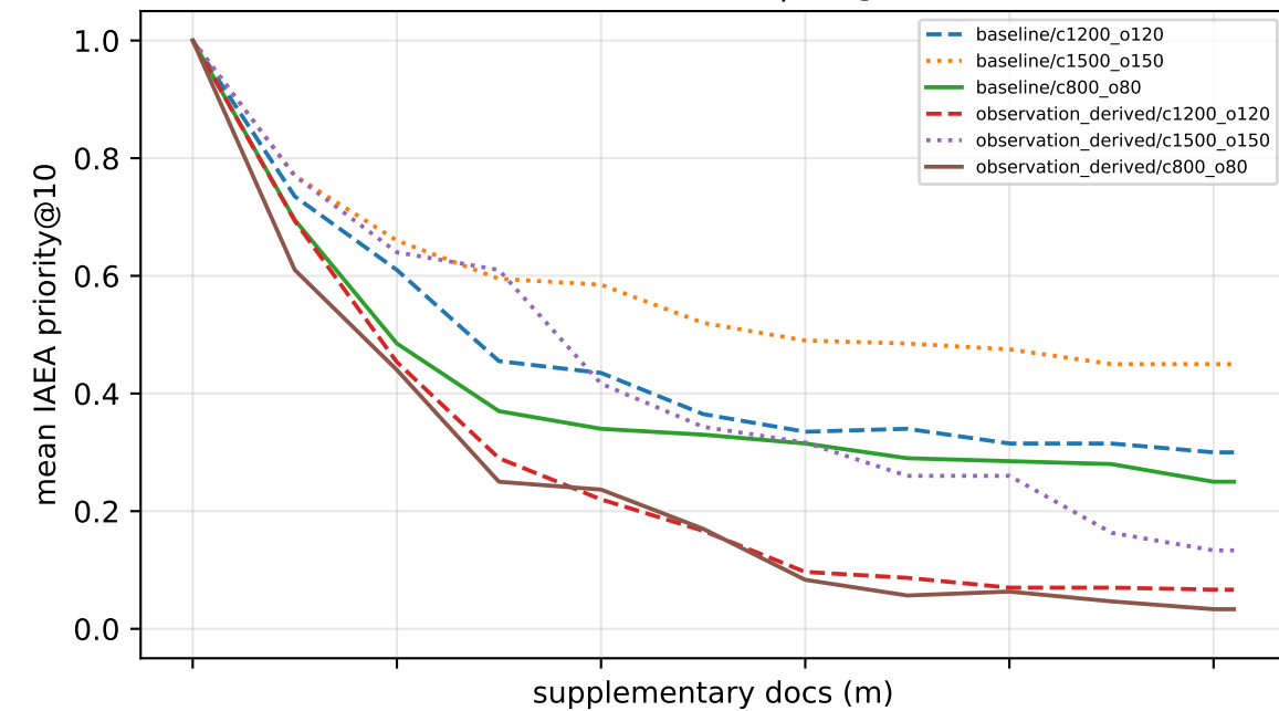
multi-MiniLM-L12-v2 | lang=zh
