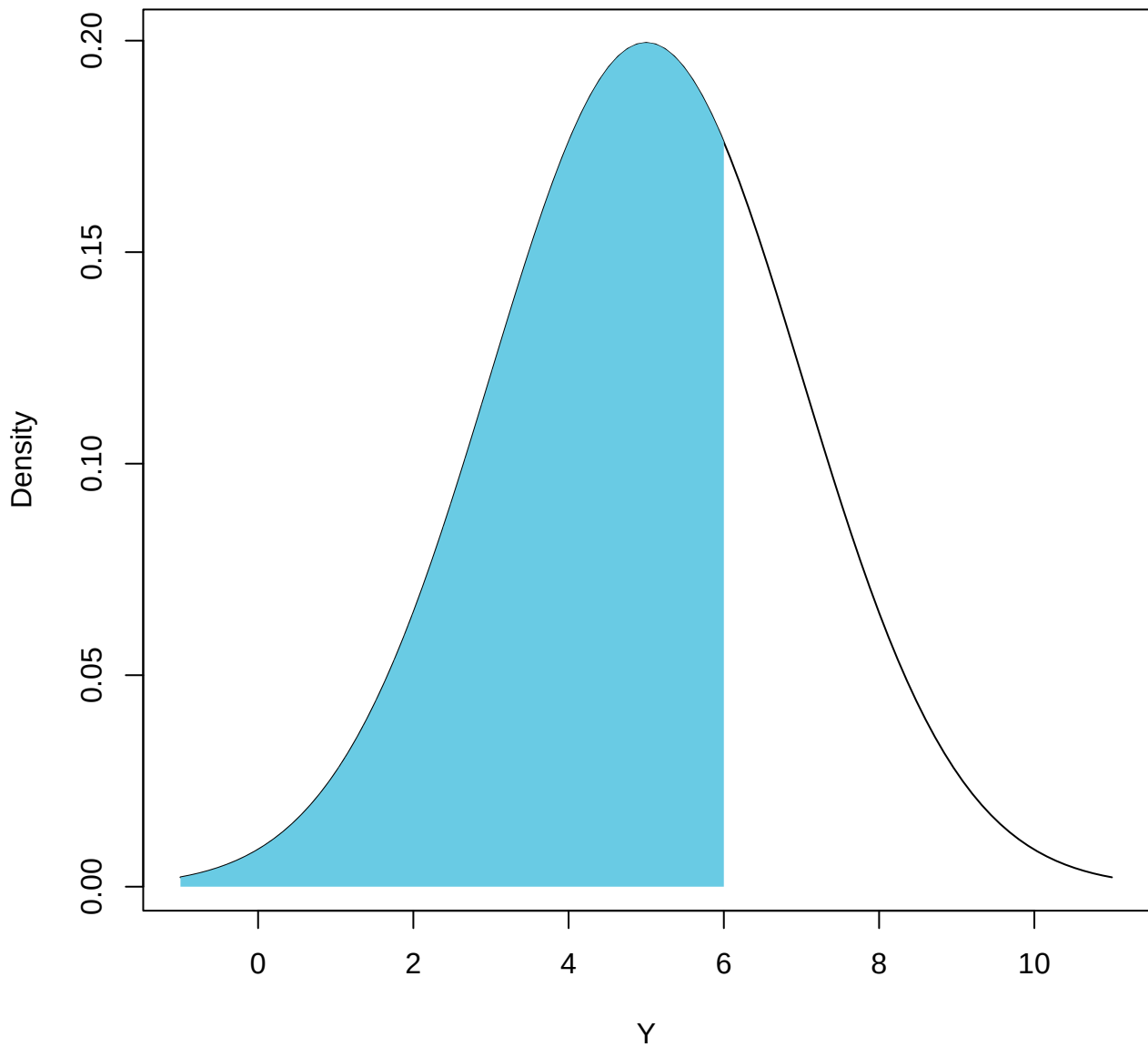
Normal Distribution N(5,4)
