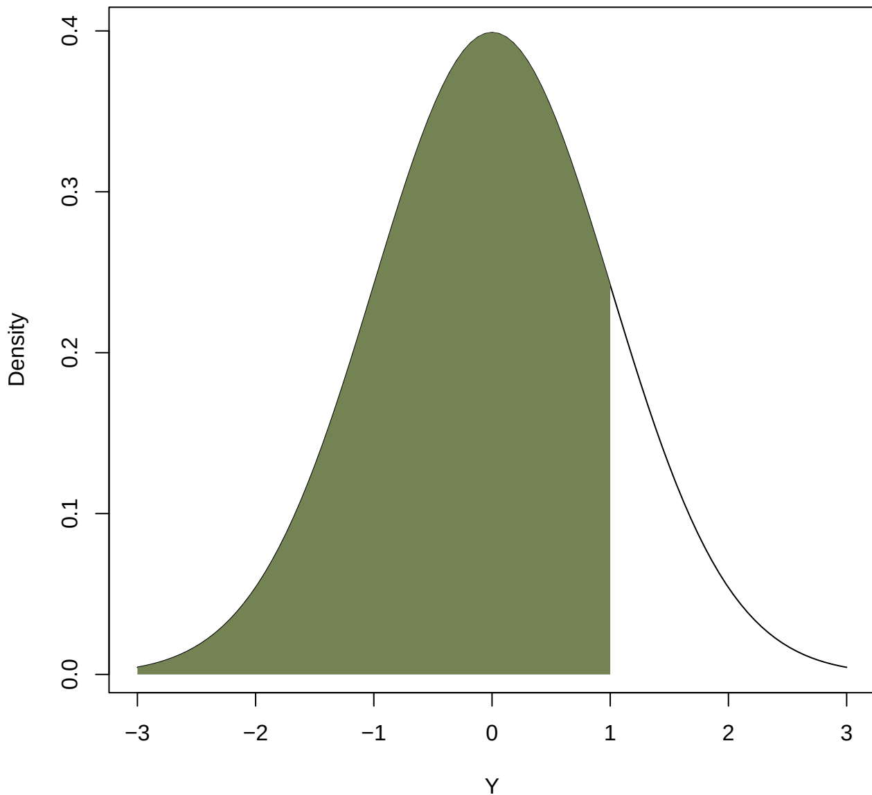
Normal Distribution N(0,1)
